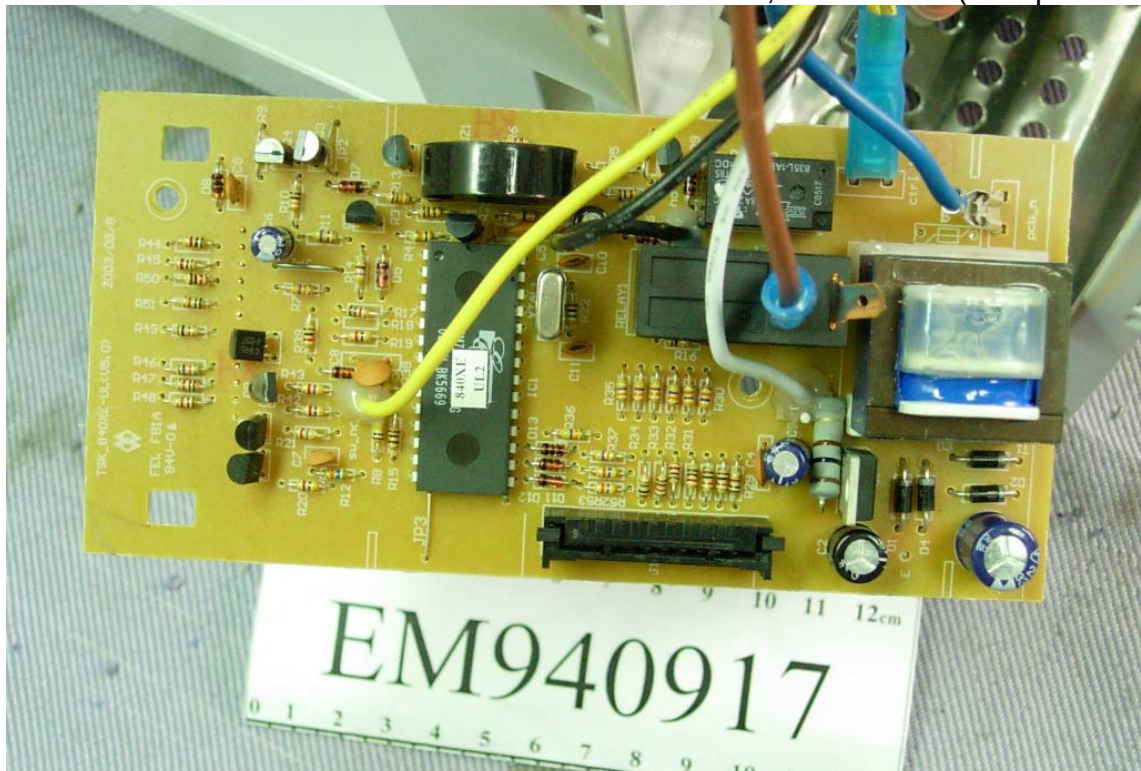
Photo 47 M/N TSK-8402EMM, Main Board (Component Side)
