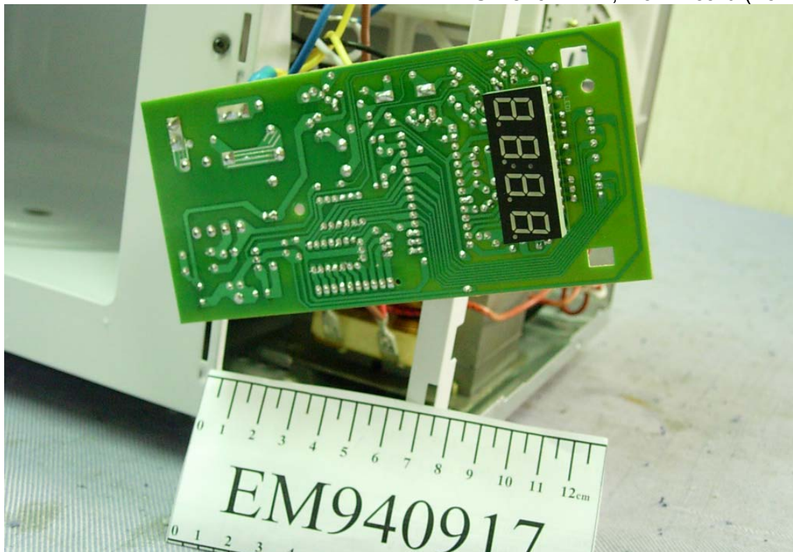
Photo 48 M/N TSK-8402EMM, Main Board (Foil Side)
