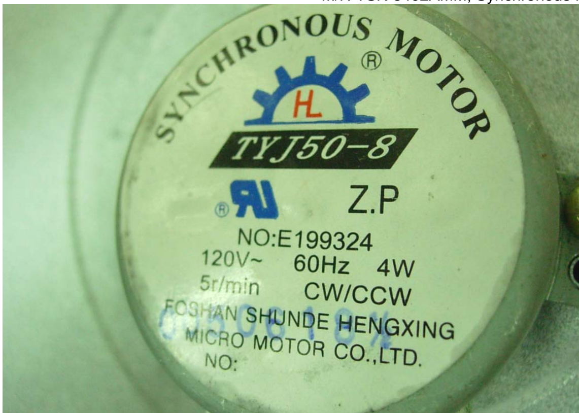
Photo 28 M/N TSK-8402AMM, Synchronous Motor
