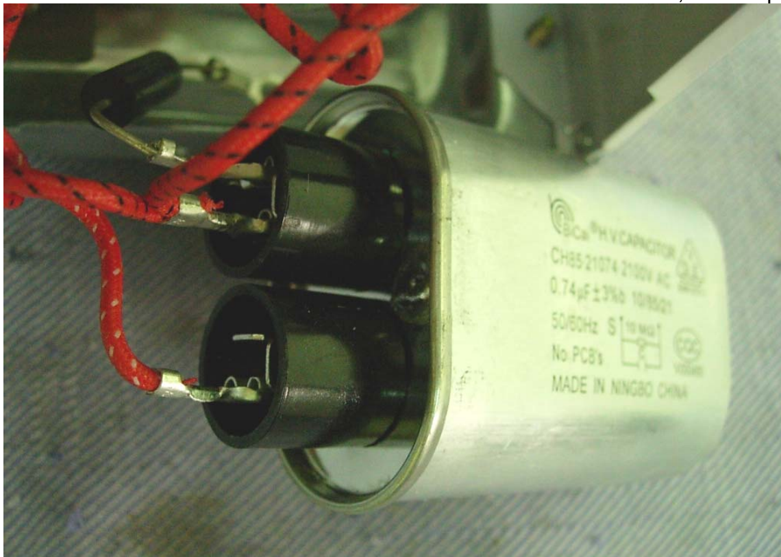
Photo 19 M/N TSK-8402AMM, H.V. Capacitor
