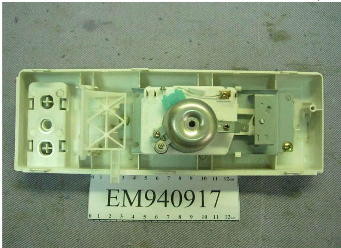
Photo 24 M/N TSK-8402AMM, Controller
