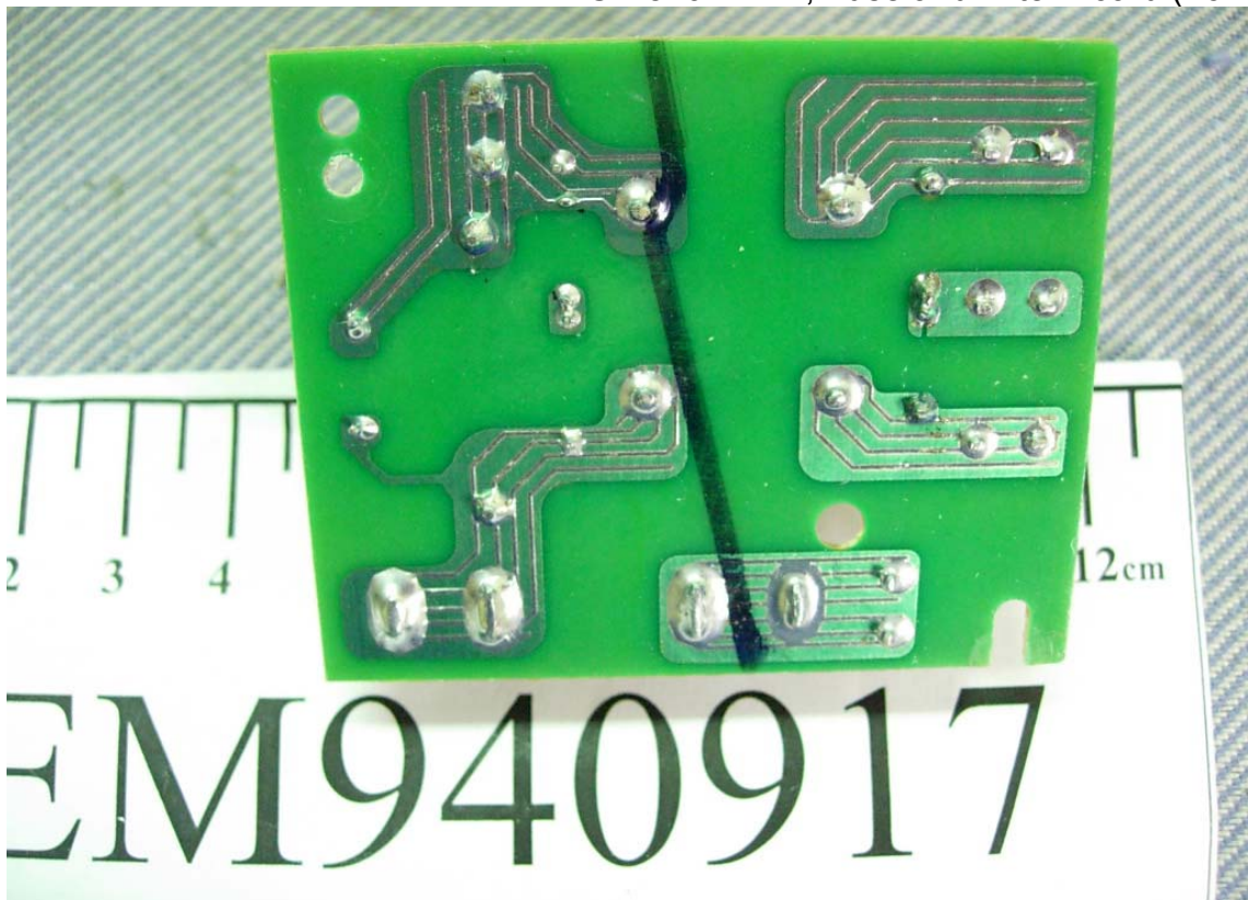
Photo 46 M/N TSK-8402EMM, Fuse and Filter Board (Foil Side)
