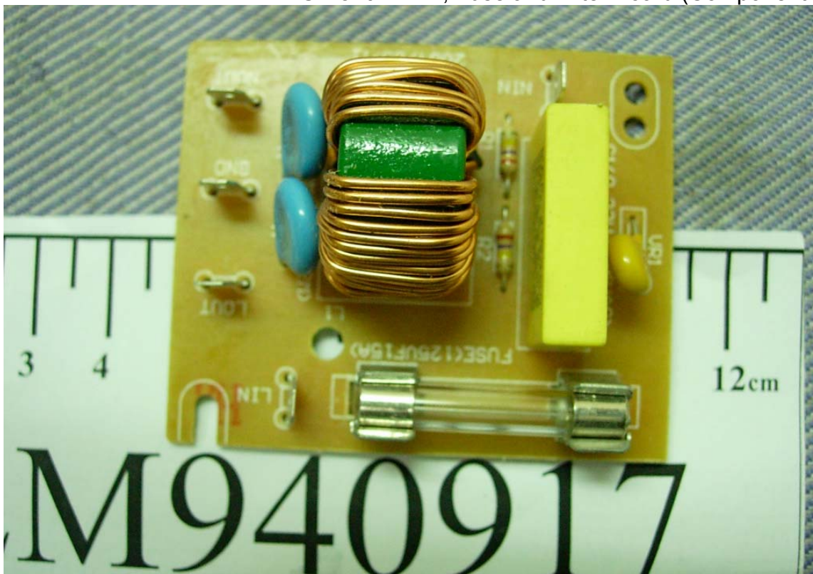
Photo 22 M/N TSK-8402AMM, Fuse and Filter Board (Component Side)
