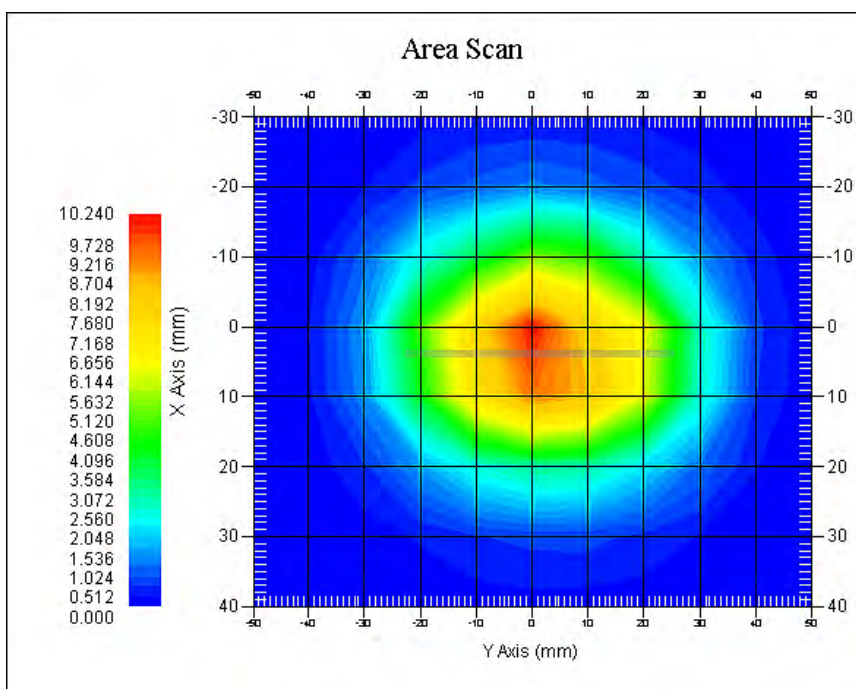
1750 MHz System Validation with Body Tissue
