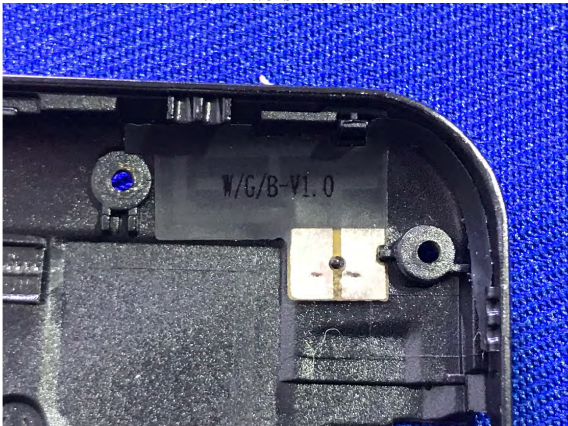
BT&WIFI&GPS Antenna View
