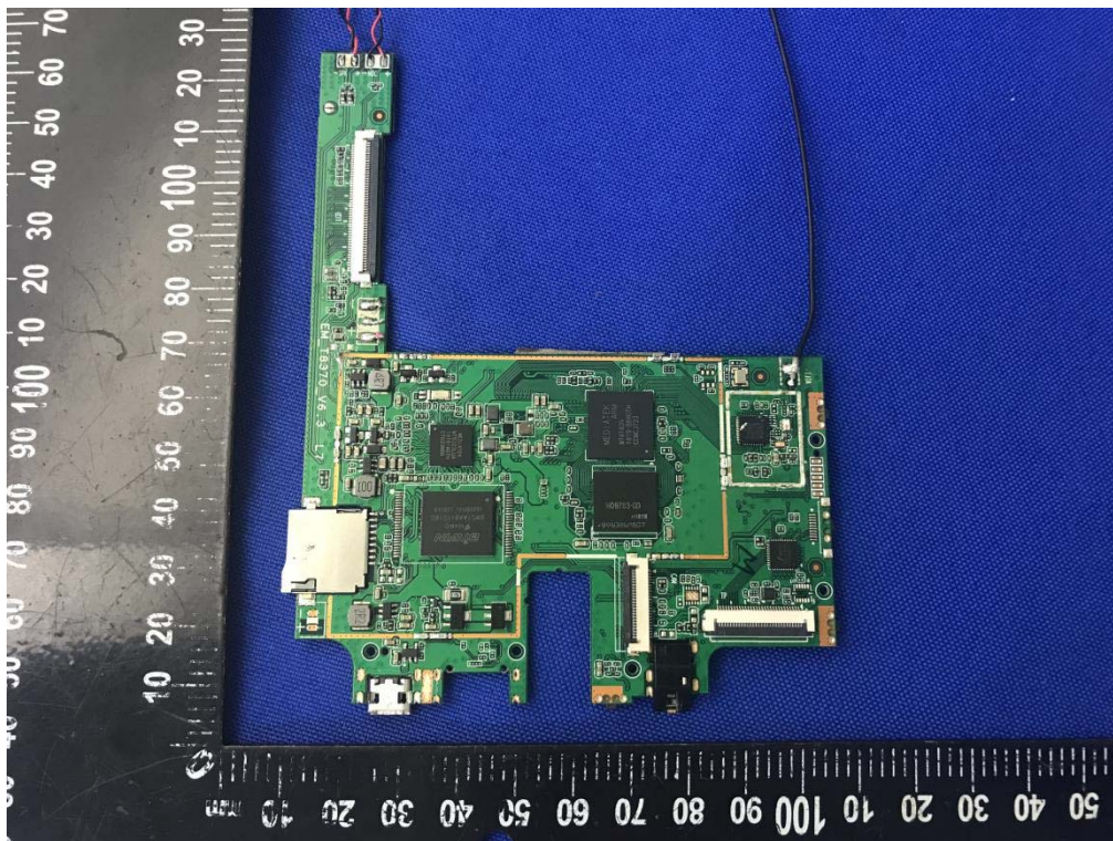
MAIN BOARD TOP VIEW (WITHOUT SHIELDING) (Configuration C)
