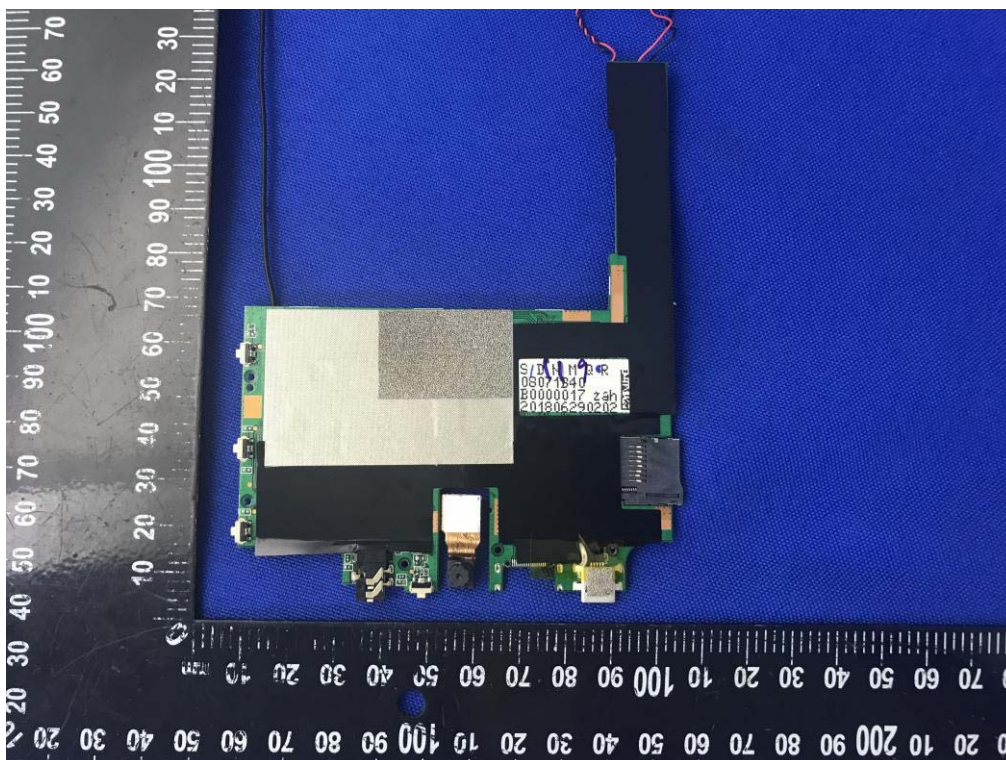
MAIN BOARD REAR VIEW (WITH SHIELDING) (Configuration D)
