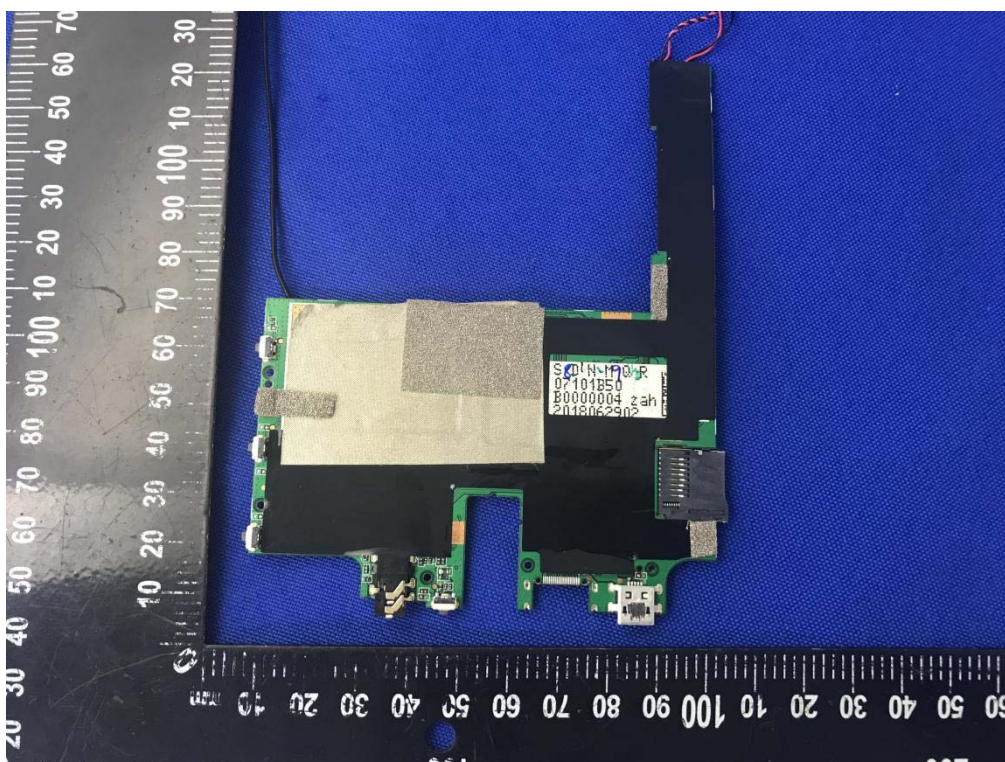
MAIN BOARD REAR VIEW (WITH SHIELDING) (Configuration C)
