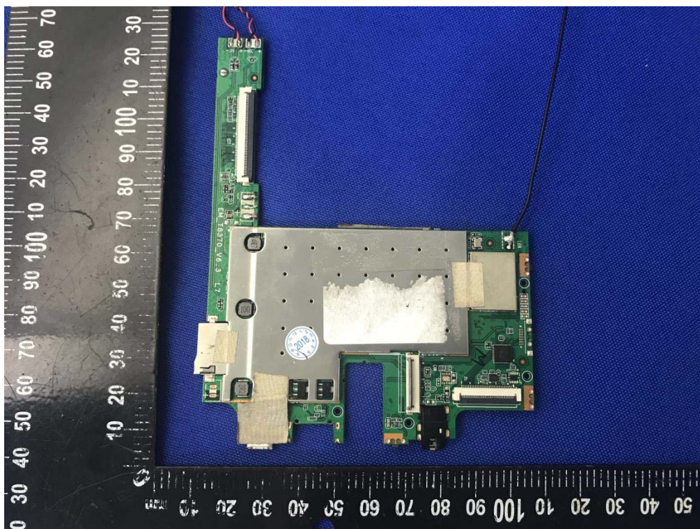
MAIN BOARD TOP VIEW (WITH SHIELDING) (Configuration C)
