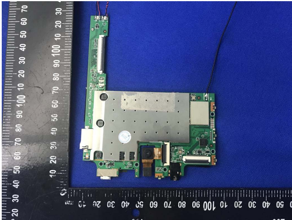
MAIN BOARD TOP VIEW (WITH SHIELDING) (Configuration D)
