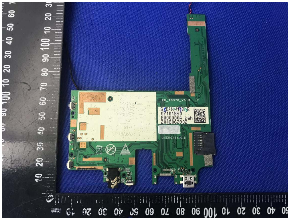
MAIN BOARD REAR VIEW (WITHOUT SHIELDING) (Configuration C)
