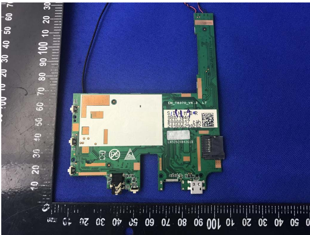
MAIN BOARD REAR VIEW (WITHOUT SHIELDING) (Configuration D)
