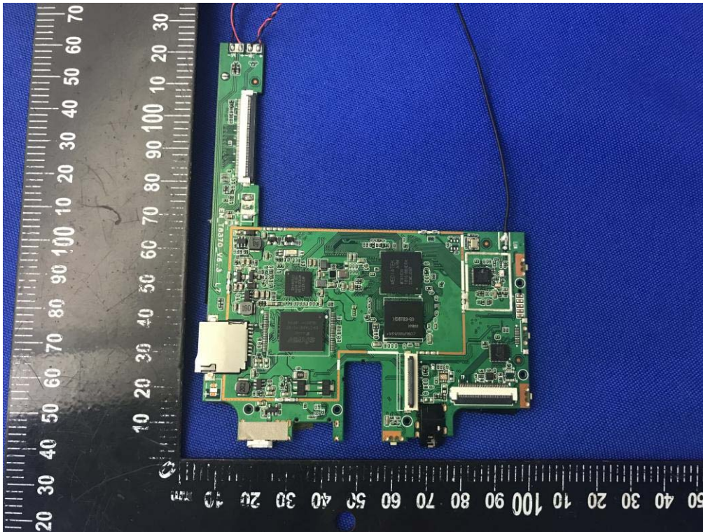
MAIN BOARD TOP VIEW (WITHOUT SHIELDING) (Configuration D)
