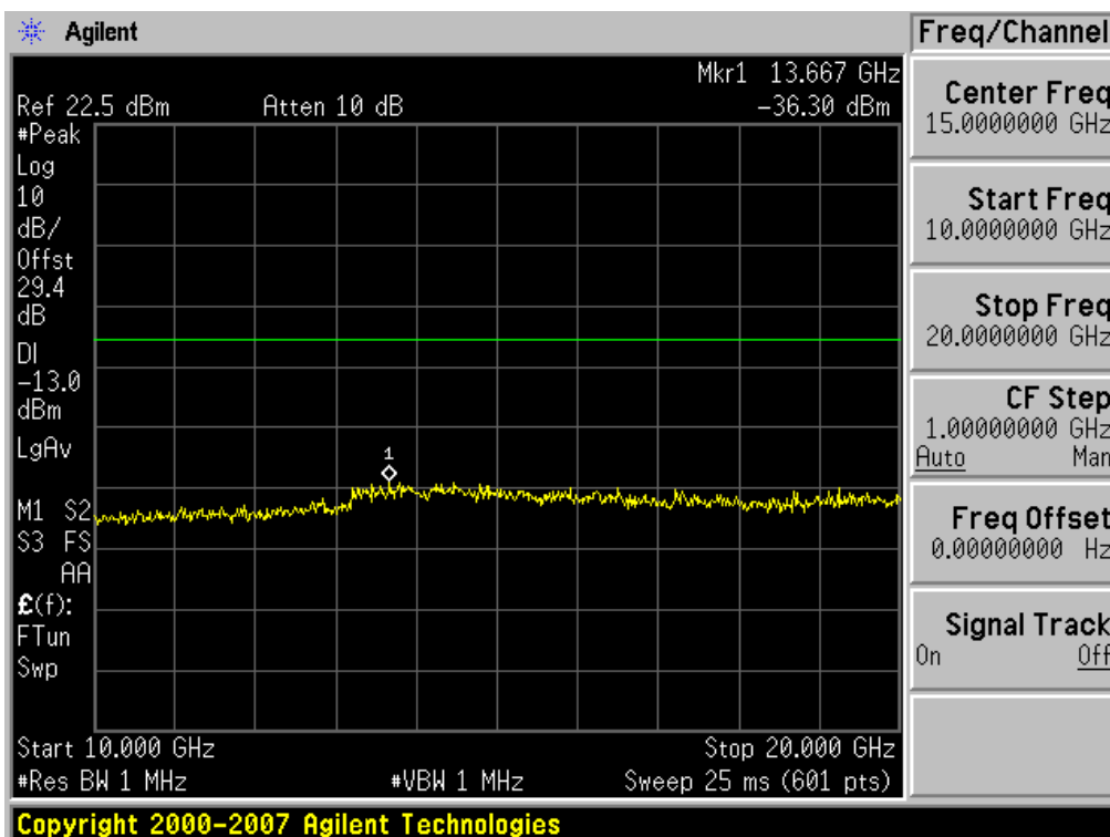
Conducted Spurious Plot (5 MHz QPSK - RB Size 25, RB Offset 0 - High Channel)-2
