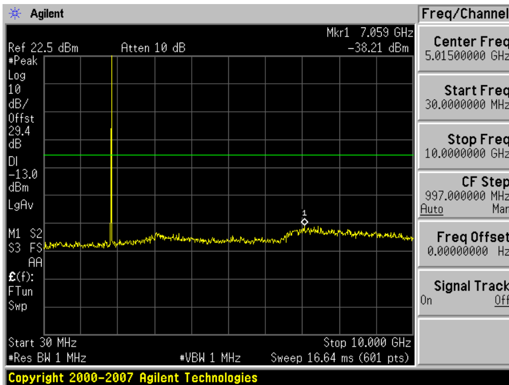
Conducted Spurious Plot (5 MHz QPSK - RB Size 25, RB Offset 0 - Low Channel)-2
