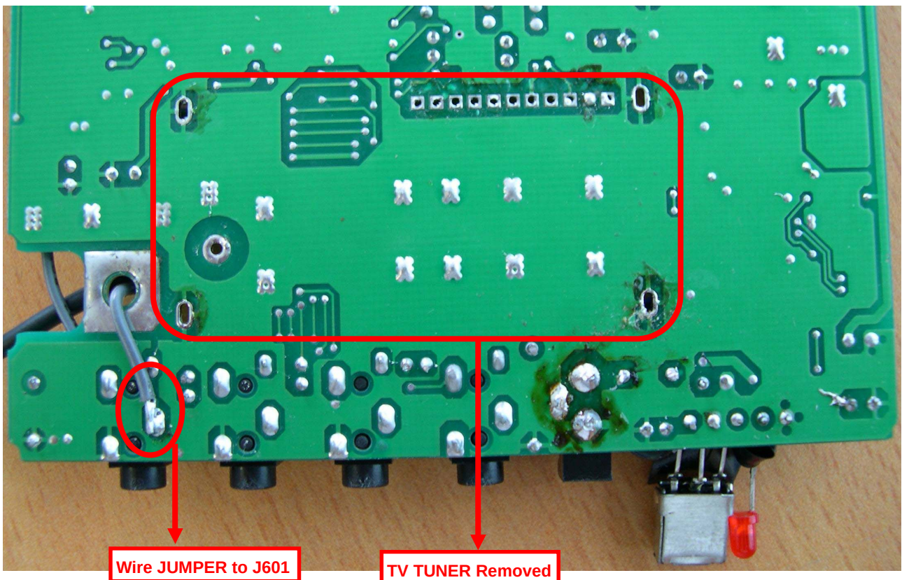
<Photograph 10: Internal rear view of the JYT-7000M>
