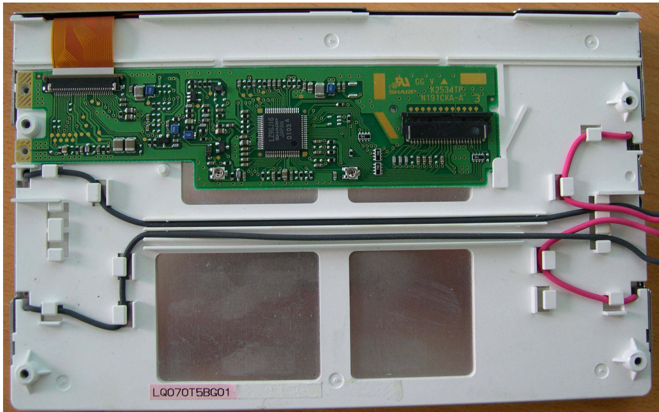
<Photograph 4: Rear view of the LCD panel>
