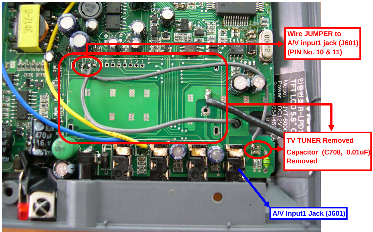
&lt;Photograph 8: Internal front view of the JYT-7000M&gt;
