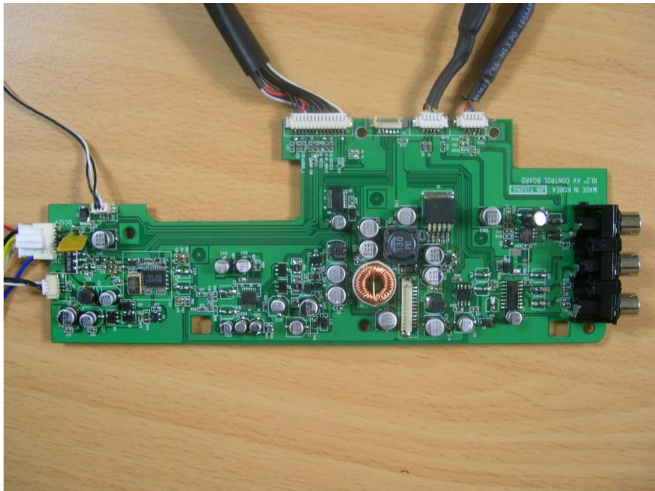
<Photograph 2: Front View-AV Board>
