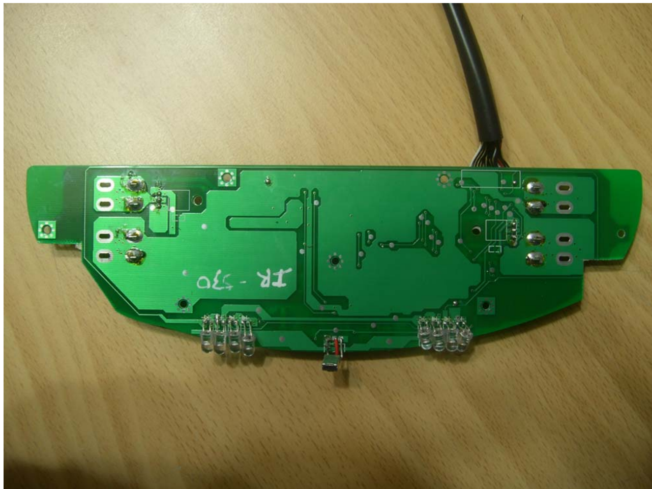
<Photograph 5: Rear View-Control Board >
