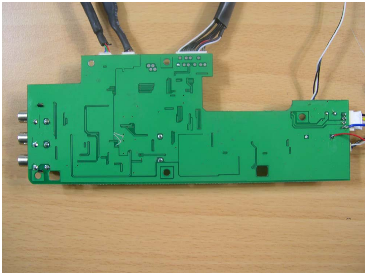
<Photograph 3: Rear View-AV Board >
