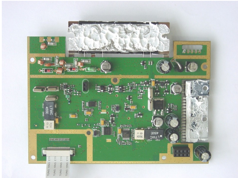
RF PCB
