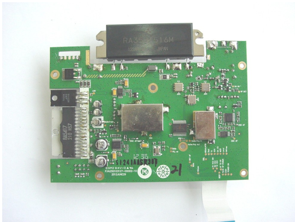
RF PCB
