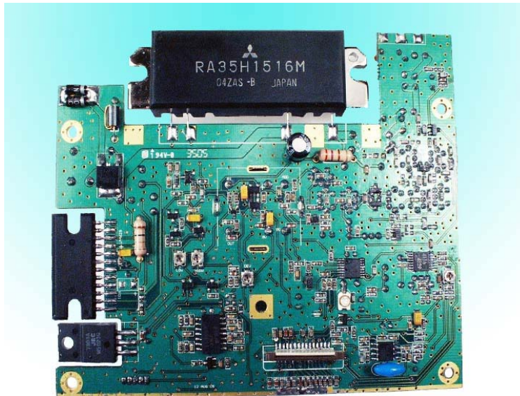
RF UNIT – TOP VIEW
