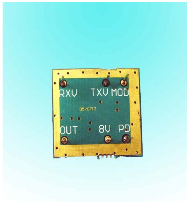
VCO UNIT – TOP VIEW
