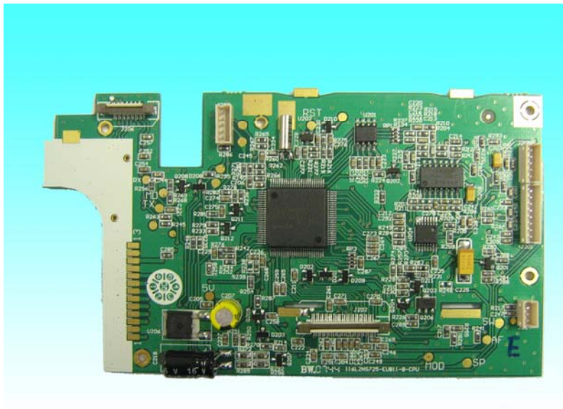
CPU UNIT – TOP VIEW
