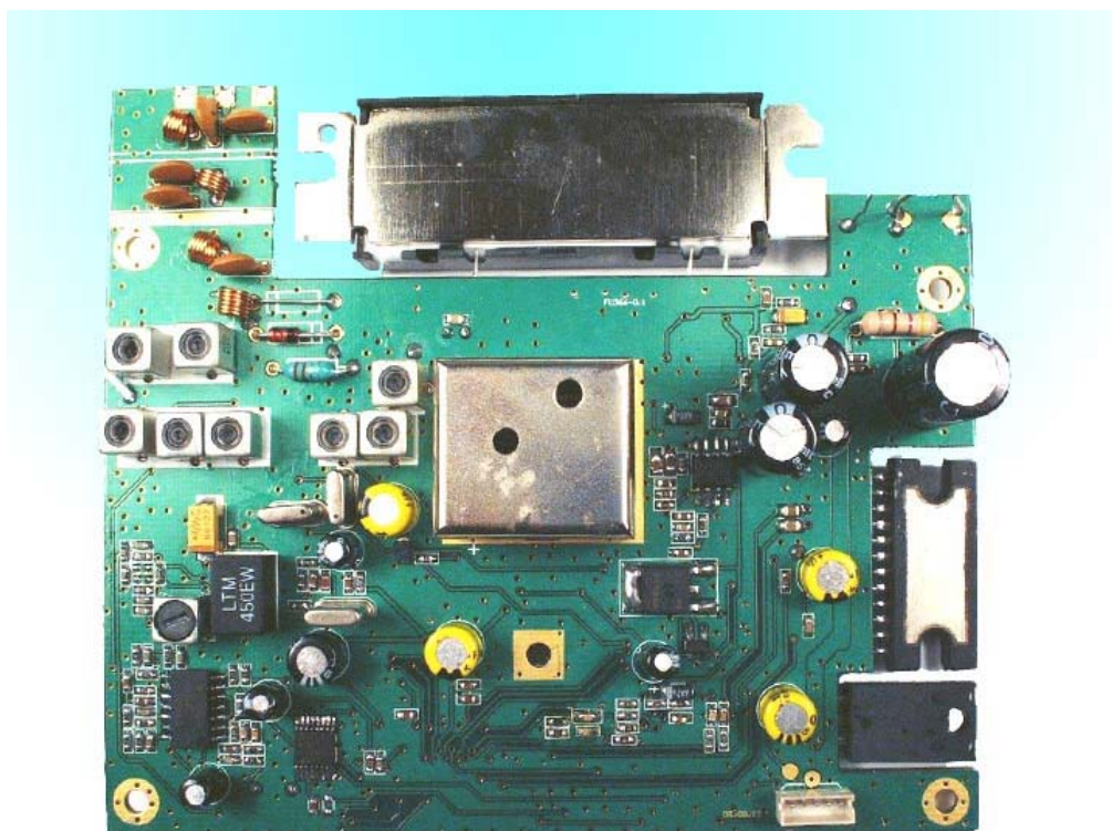
RF UNIT – TOP VIEW
