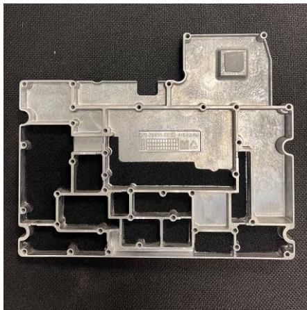
RF Shield
