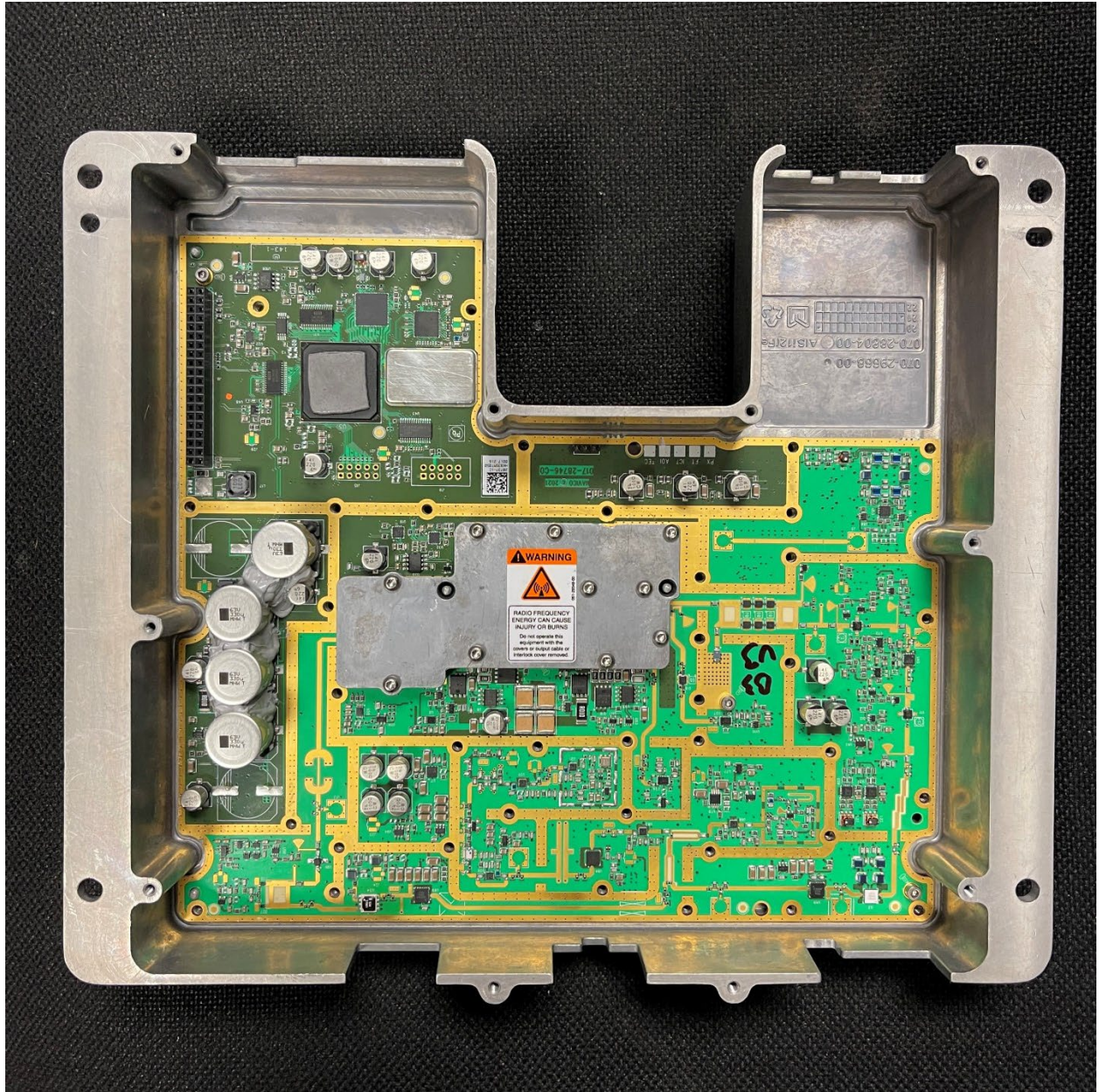
PA CIVER OVER RF PCBA
