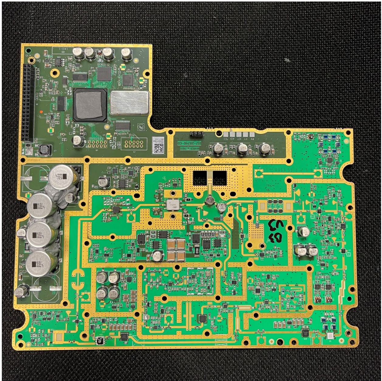
RF PCB - UNDERSIDE
