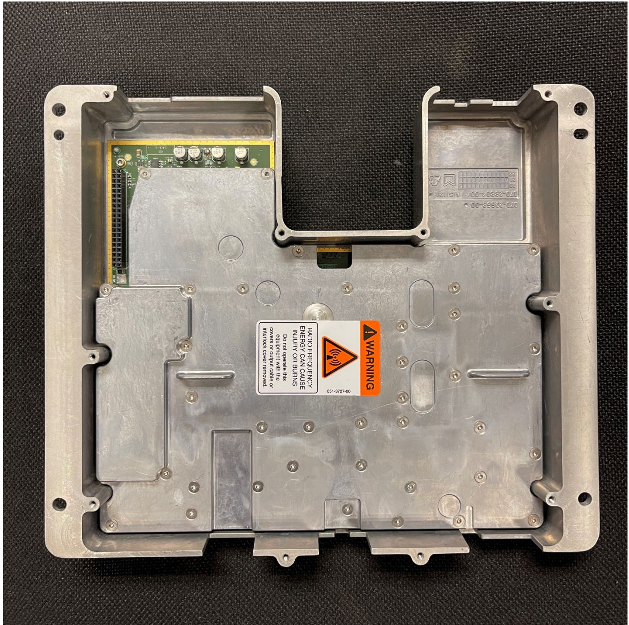
RF SHIELD OVER PA COVER
