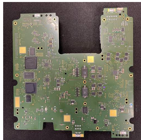
CPU PCBA - underside
