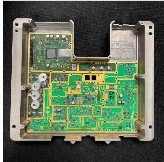
RF Housing + RF PCBA
