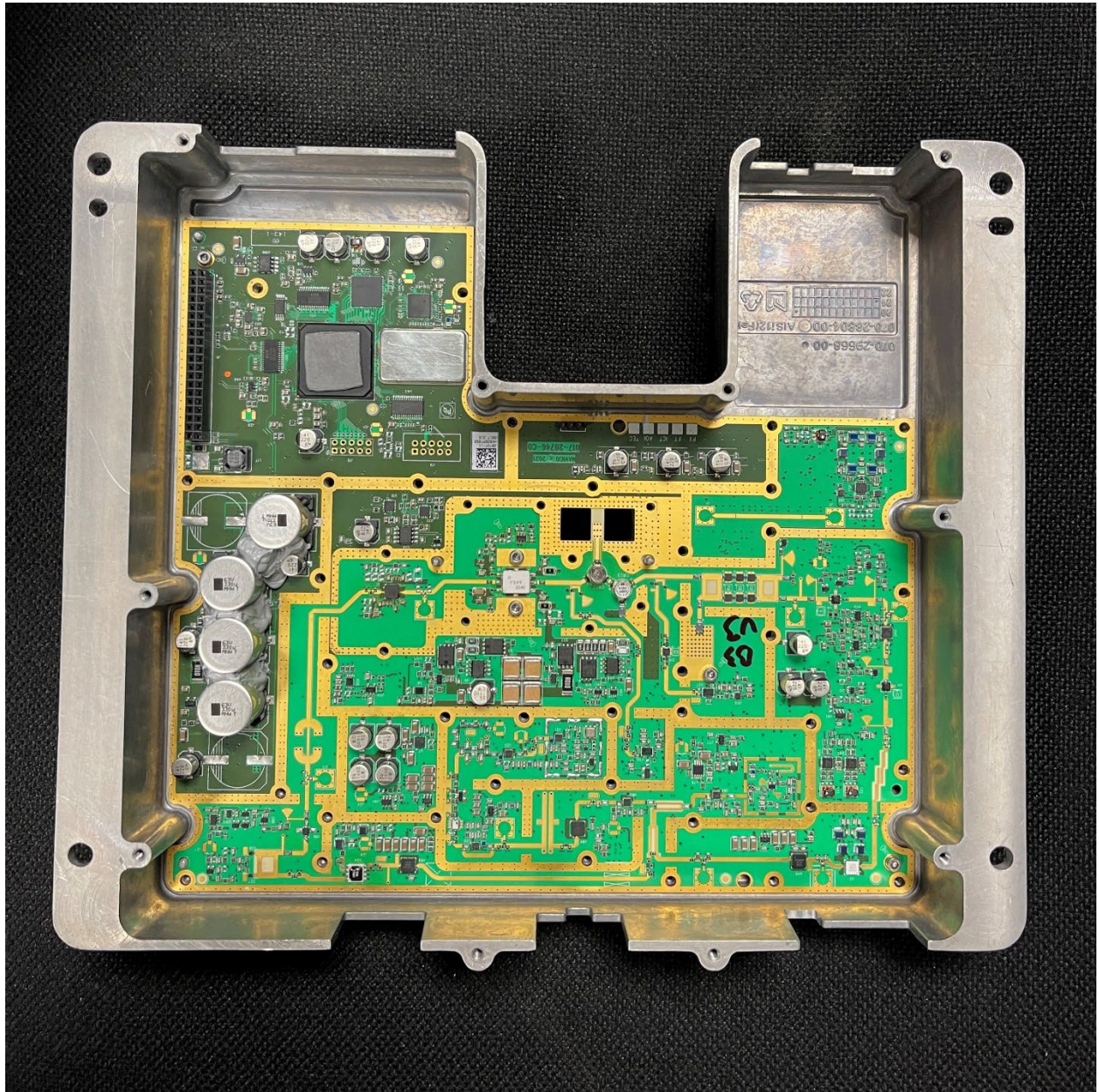
RF HOUSE + RF PCBA
