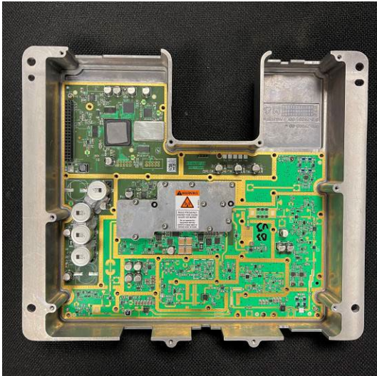
PA Cover over RF PCBA
