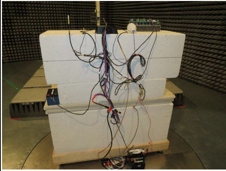
Test setup-3
