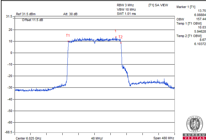
802.11ax (HE160) Beamforming / Chain 0 : CH 15
