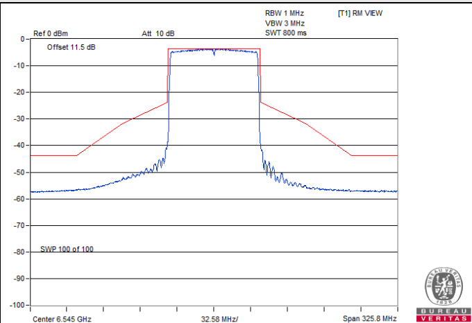
802.11ax (HE80) Beamforming / Chain 3 : CH 119
