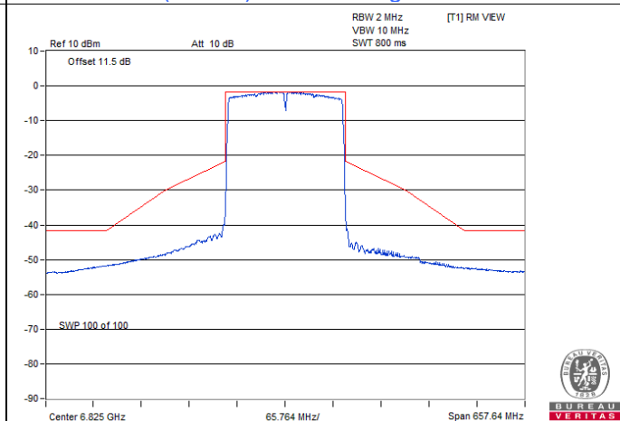
802.11ax (HE160) Beamforming / Chain 0 : CH 175
