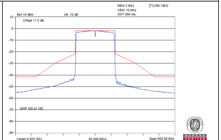
802.11ax (HE160) Beamforming / Chain 2 : CH 175
