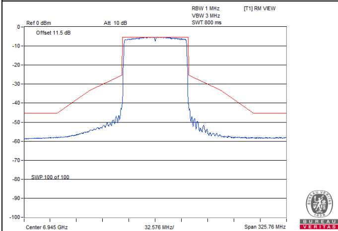
802.11ax (HE80) Beamforming / Chain 1 : CH 199
