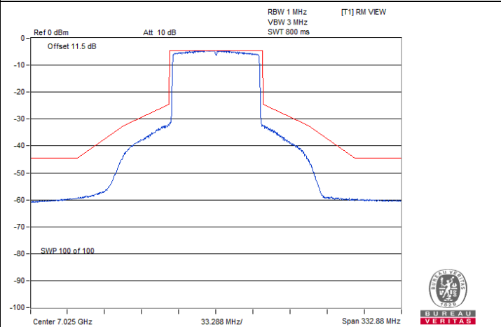
802.11ax (HE80) Beamforming / Chain 1 : CH 215
