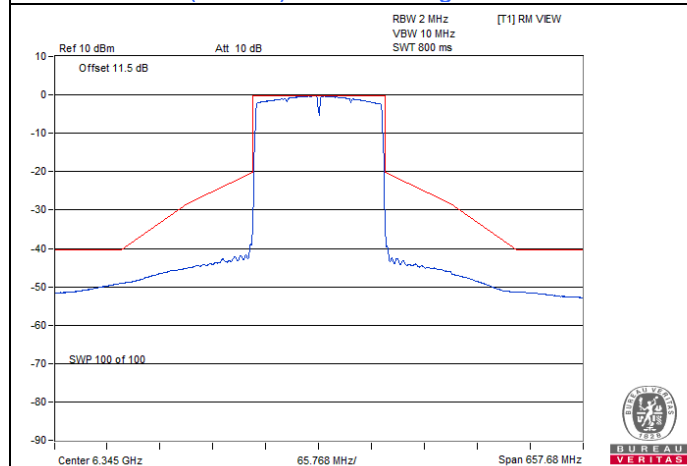
802.11ax (HE160) Beamforming / Chain 0 : CH 79
