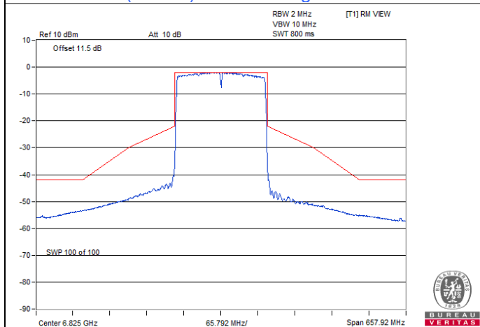
802.11ax (HE160) Beamforming / Chain 3 : CH 175
