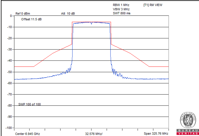
802.11ax (HE80) Beamforming / Chain 3 : CH 199
