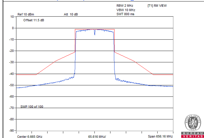
802.11ax (HE160) Beamforming / Chain 0 : CH 143
