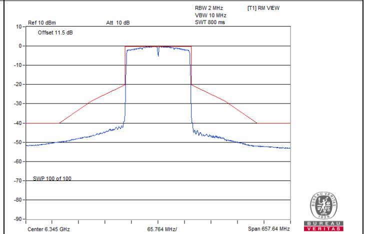
802.11ax (HE160) Beamforming / Chain 1 : CH 79
