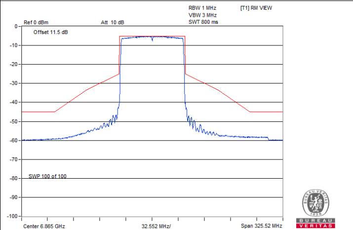
802.11ax (HE80) Beamforming / Chain 1 : CH 183
