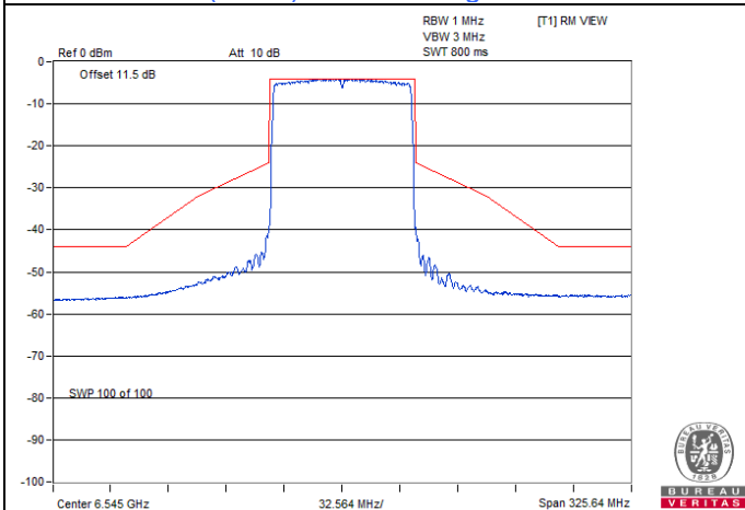
802.11ax (HE80) Beamforming / Chain 2 : CH 119
