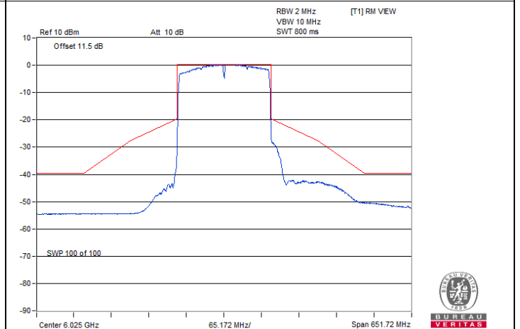
802.11ax (HE160) Beamforming / Chain 3 : CH 15
