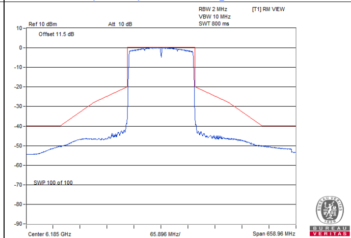
802.11ax (HE160) Beamforming / Chain 2 : CH 47
