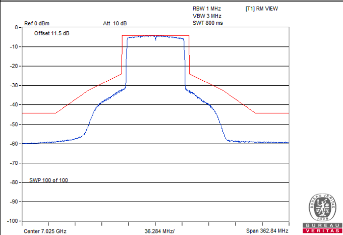
802.11ax (HE80) Beamforming / Chain 3 : CH 215
