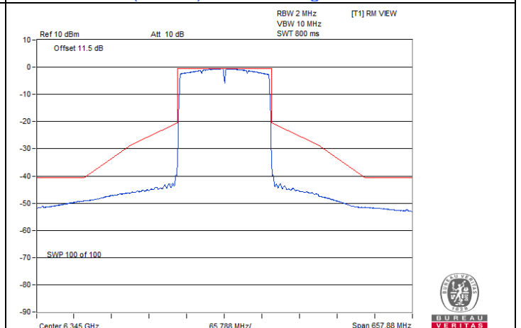
802.11ax (HE160) Beamforming / Chain 3 : CH 79
