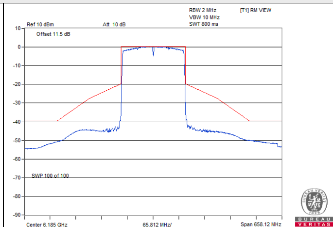
802.11ax (HE160) Beamforming / Chain 0 : CH 47
