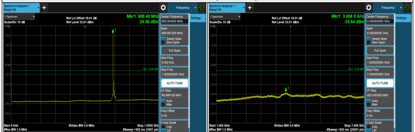
Channel 138600 (693 MHz)
