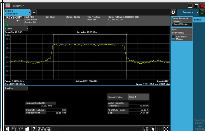
BPSK CH 656000 (3840 MHz)
