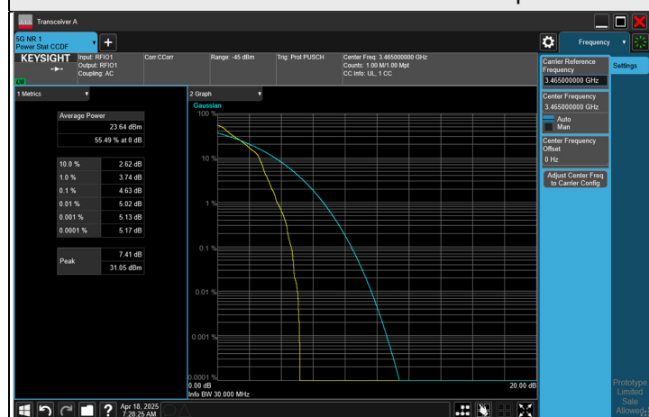
BPSK CH 631000 (3465 MHz)
