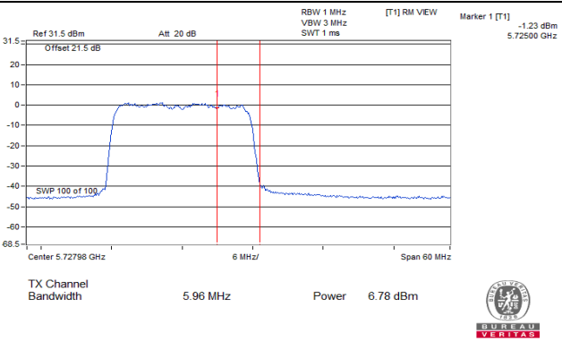
802.11ax (HE20)_Chain 1 / CH144 (U-NII-3 Band)
