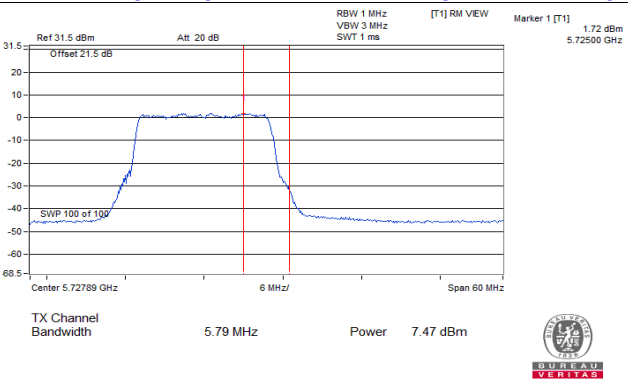
802.11ax (HE20)_Chain 3 / CH144 (U-NII-3 Band)
