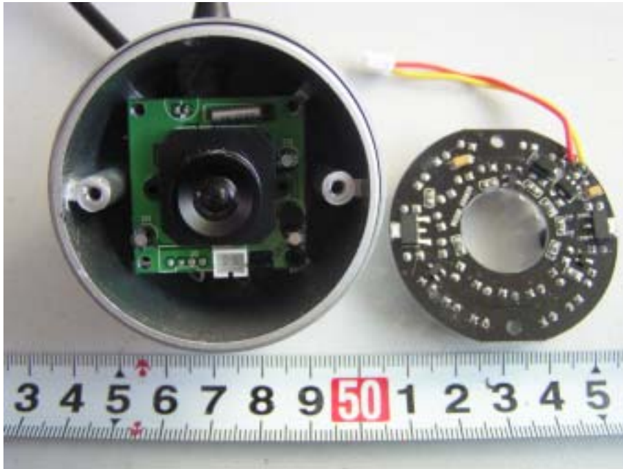
EUT-Inside View (3)
