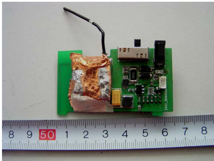
EUT-RF board Bottom View (1)
