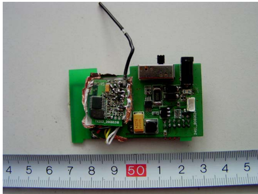
EUT-RF board Bottom View (2)
