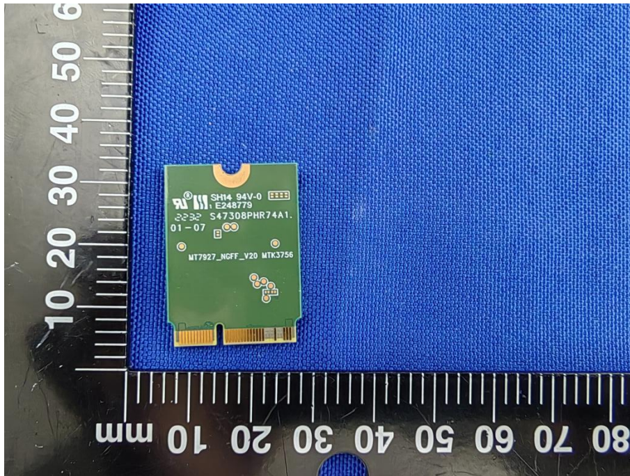
RF MODULE REAR VIEW-MT7927
