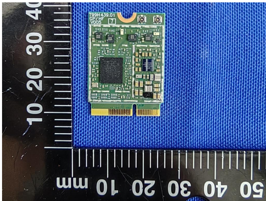
RF MODULE TOP(WITHOUT SHIELDING) VIEW-MT7927
