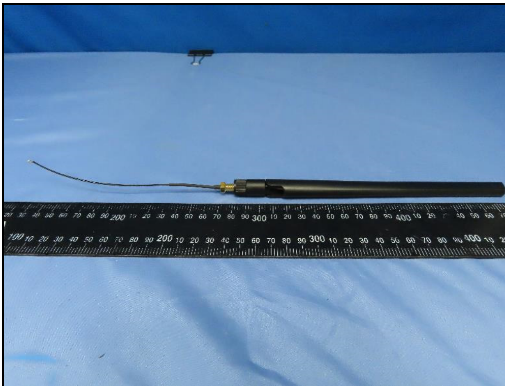
Ant. Set 6 (Brand: PSA / Model: RFPCA460632IMMB701)
