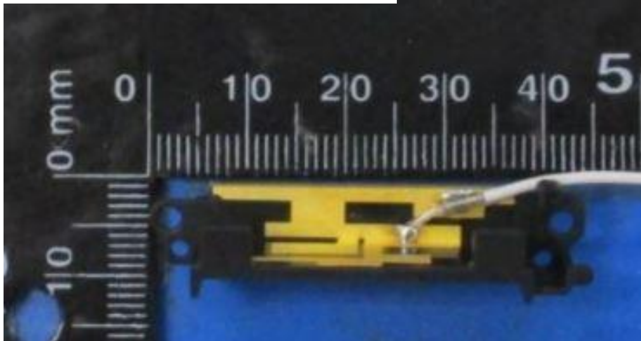
WLAN Main Antenna for Wistron NeWeb Corporation
