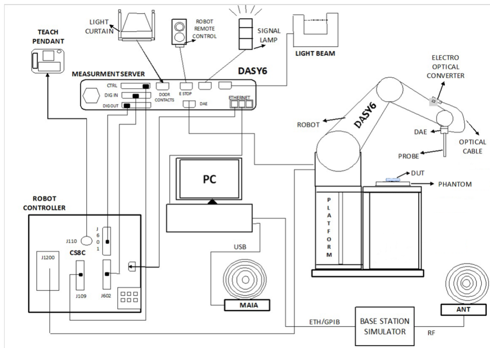
Fig-5.1 SPEAG DASY6 System Configuration
