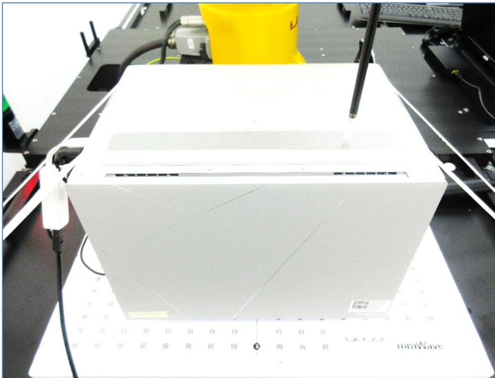
Setup for Power Density Testing (Bottom Surface of Base at 2 mm)
