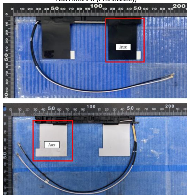
Aux Antenna (Front/Back))
