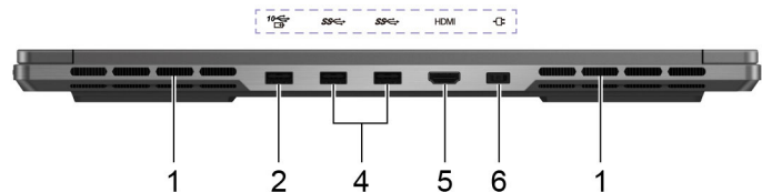
Figure 2. Rear view—Legion Slim 7 16APH8 and Lenovo Legion Slim 7 16APH8 D2
