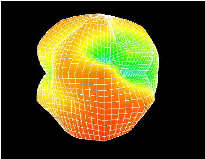
Max Antenna 3D Radiation Pattern 5150-5250 MHz
