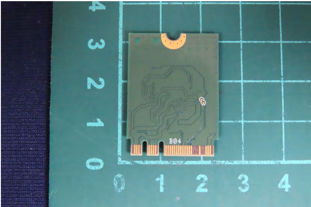
(6) EUT Photo_MT7922A22M
