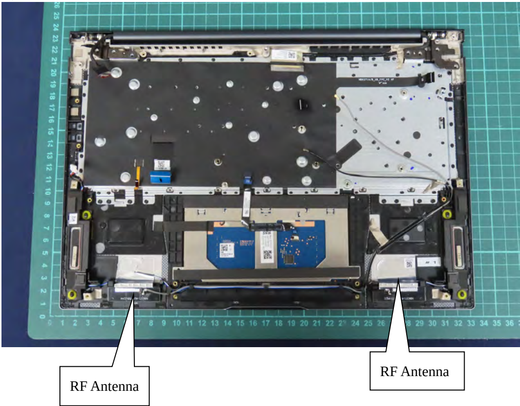
(22) EUT Photo
