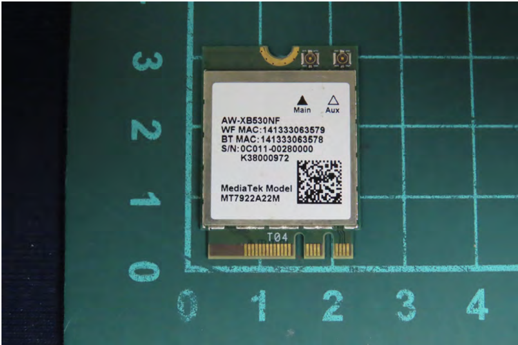
(5) EUT Photo_MT7922A22M
