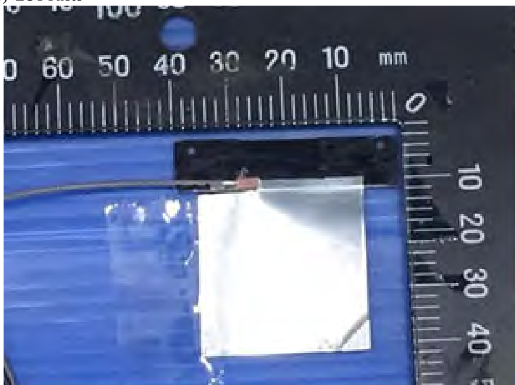
(29) EUT Photo
