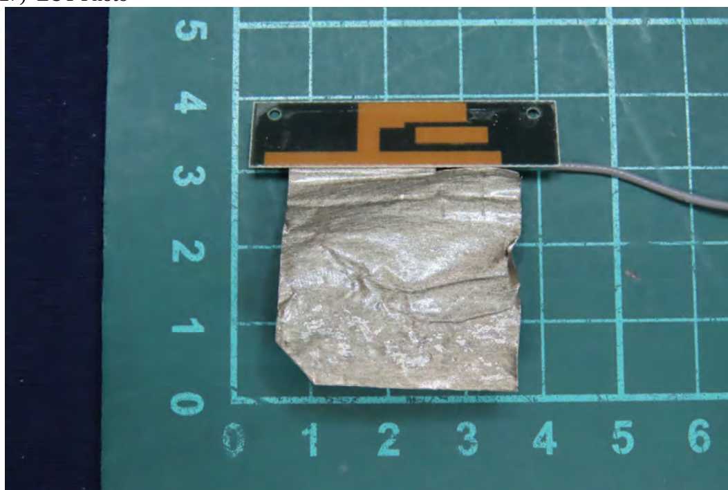
(27) EUT Photo
