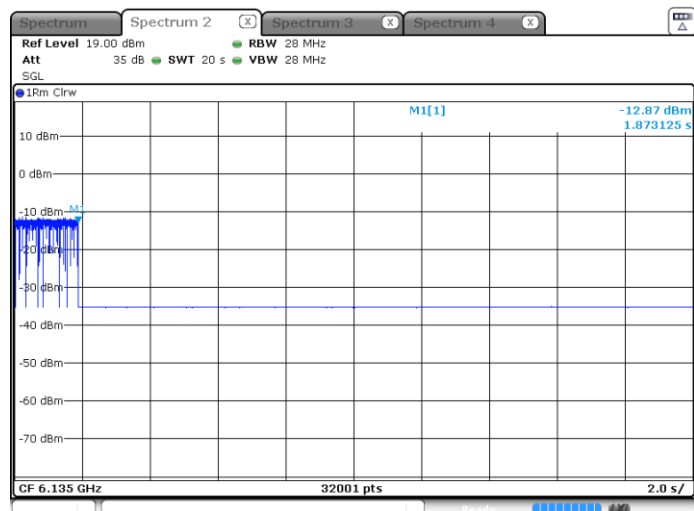
802.11ax (HE20)-Channel 37
