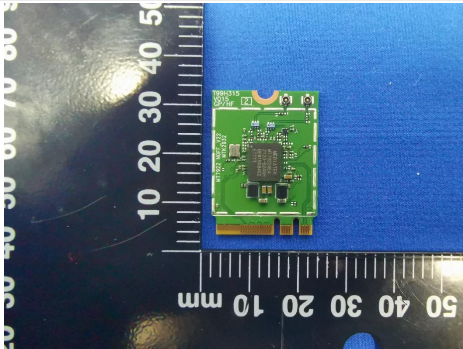
TOP SIDE VIEW OF EUT
