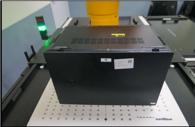
Bottom of EUT Tested at 0 mm
