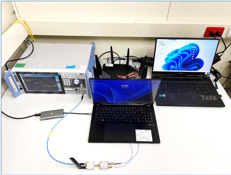
Setup for Conducted Power Testing (Test Scenario 1 and 3)
