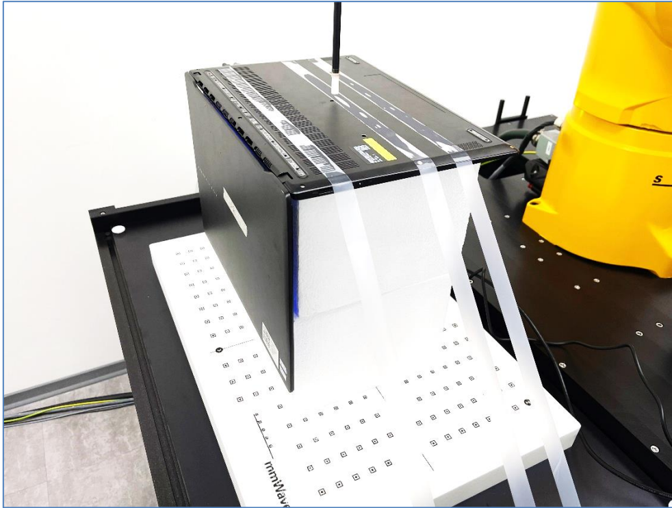
Setup for Power Density Testing (Bottom Surface at 2 mm)
