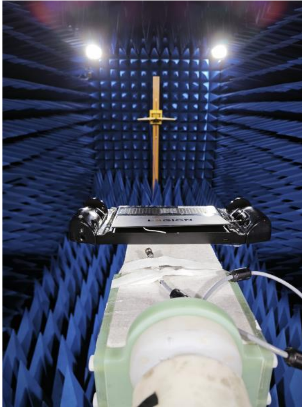
Setup photo
