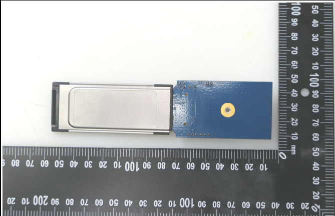
Rear Face of jig
