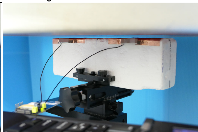
Bottom Side of EUT Tested at 5 mm
