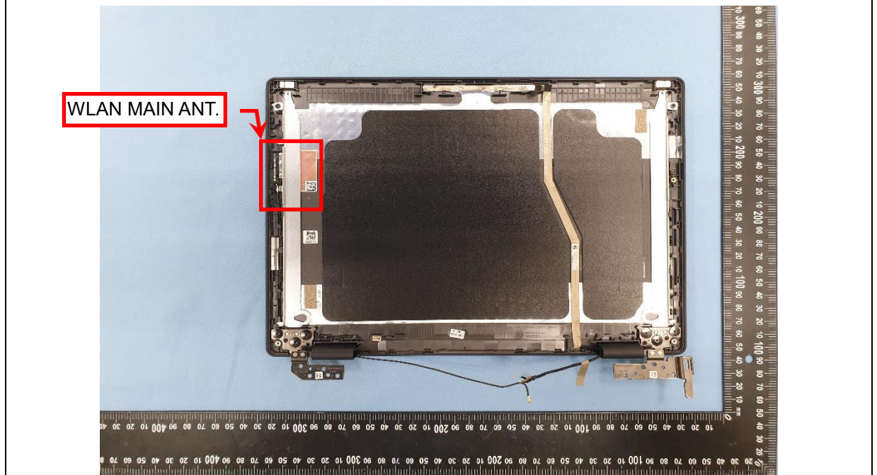
EUT Photo (35) Platform Model Number:CR1104FG, CR1104CG
