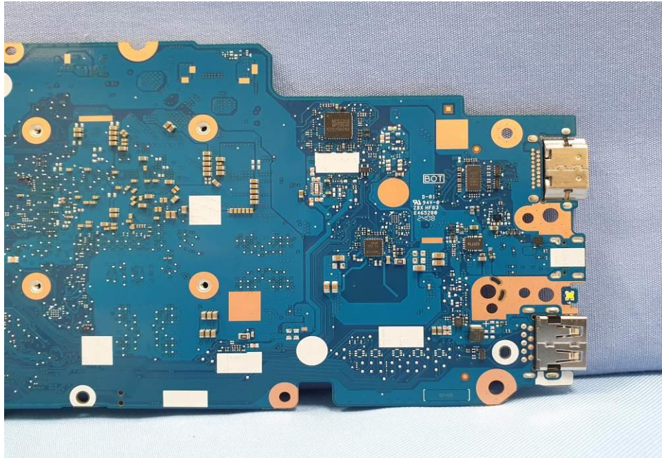
EUT Photo (34) Platform Model Number: CR1204FG, CR1204CG
