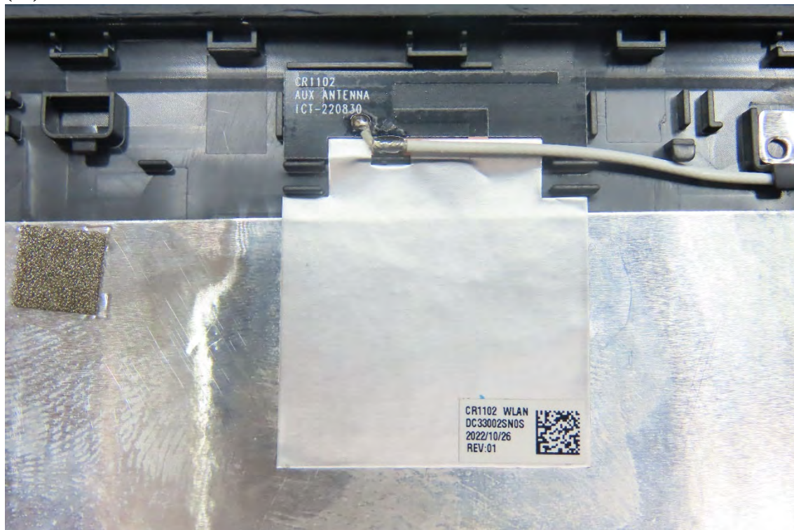
(26) EUT Photo
