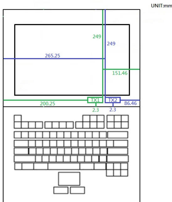
Photograph 5. Antenna position of EUT
