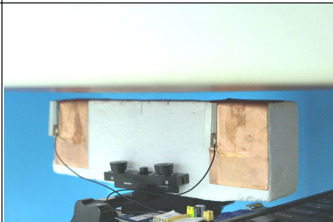
Right Side of EUT Tested at 8 mm
