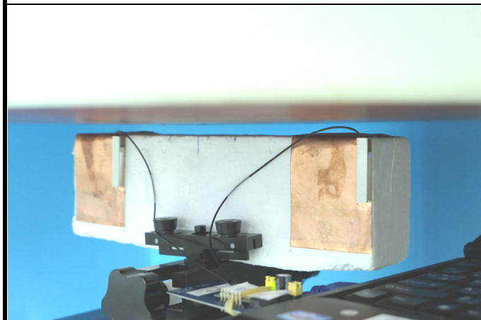
Left Side of EUT Tested at 8 mm
