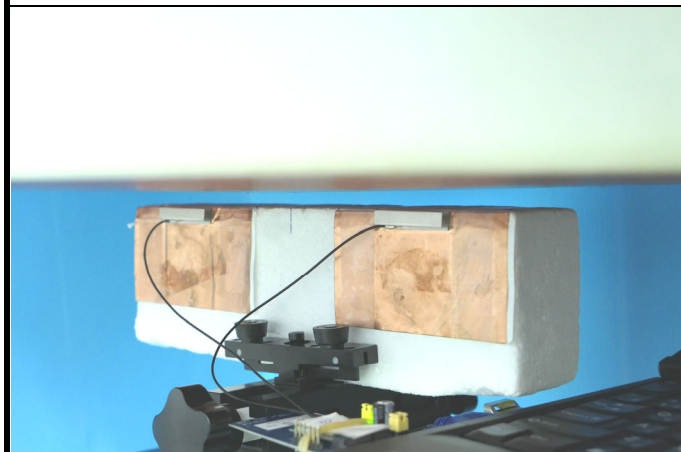
Top Side of EUT Tested at 8 mm
