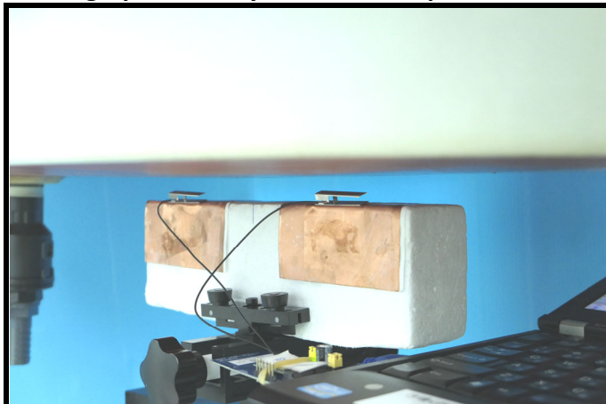
Front Face of EUT Tested at 8 mm
