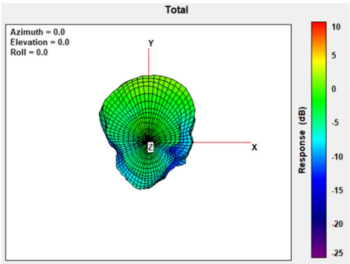
Max Antenna 3D Radiation Pattern 5150-5250 MHz
