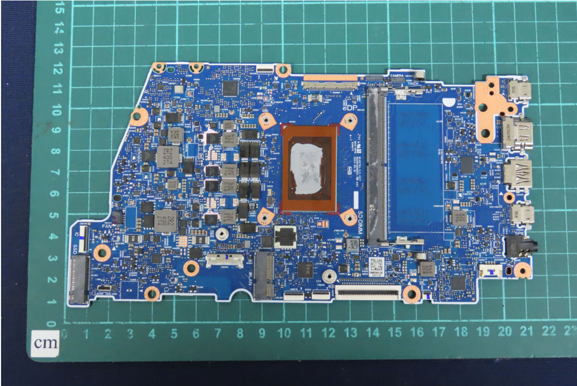
(35) EUT Photo
