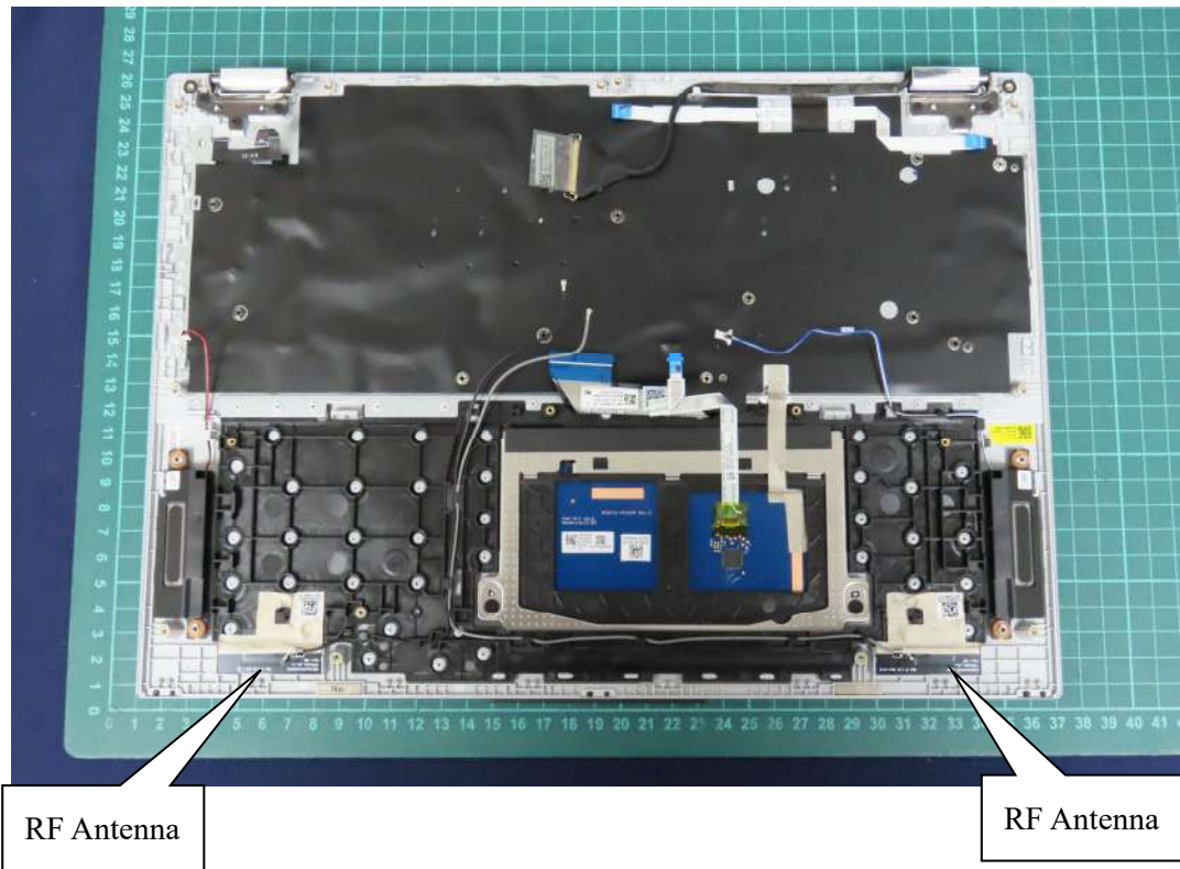
(27) EUT Photo
