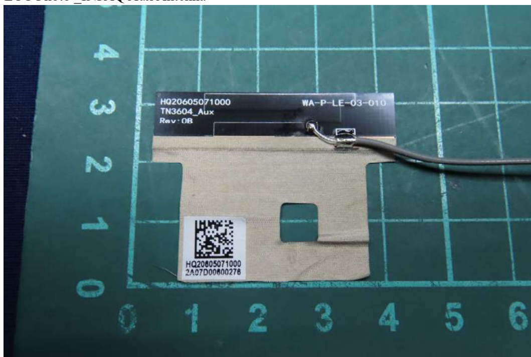
(31) EUT Photo _INPAQ Aux Antenna
