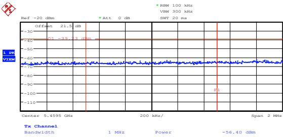
Figure 8.5-17: Peak spurious emission at 5.46 GHz on low channel, 802.11n HT40, ch1
