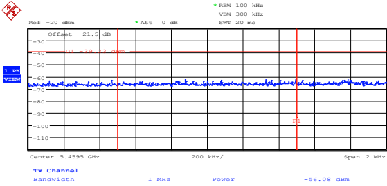
Figure 8.5-5: Peak spurious emission at 5.46 GHz on low channel, 802.11a, ch1
