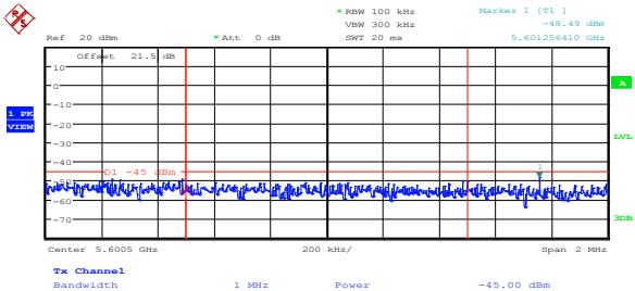
Figure 8.5-54: Upper band edge emission of the first frequency block at 5.6 GHz on mid channel, 802.11n HT40, ch1
