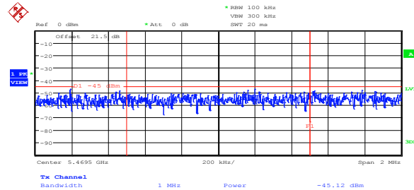
Figure 8.5-38: Lower band edge emission at 5.47 GHz on low channel, 802.11n HT20, ch1
