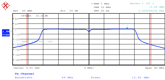
Figure 8.4-3: Output power and PSD on 802.11n HT40, sample plot
