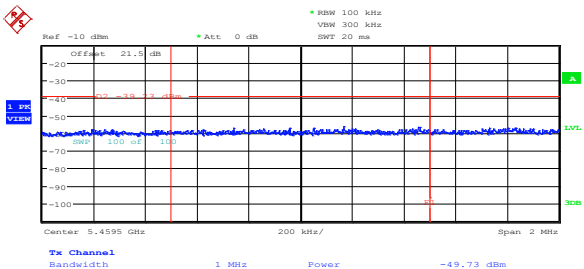
Figure 8.5-2: Peak spurious emission at 5.46 GHz on low channel, 802.11a, cho
