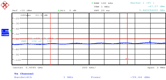
Figure 8.5-15: Average spurious emission at 5.46 GHz on low channel, 802.11n HT40, cho
