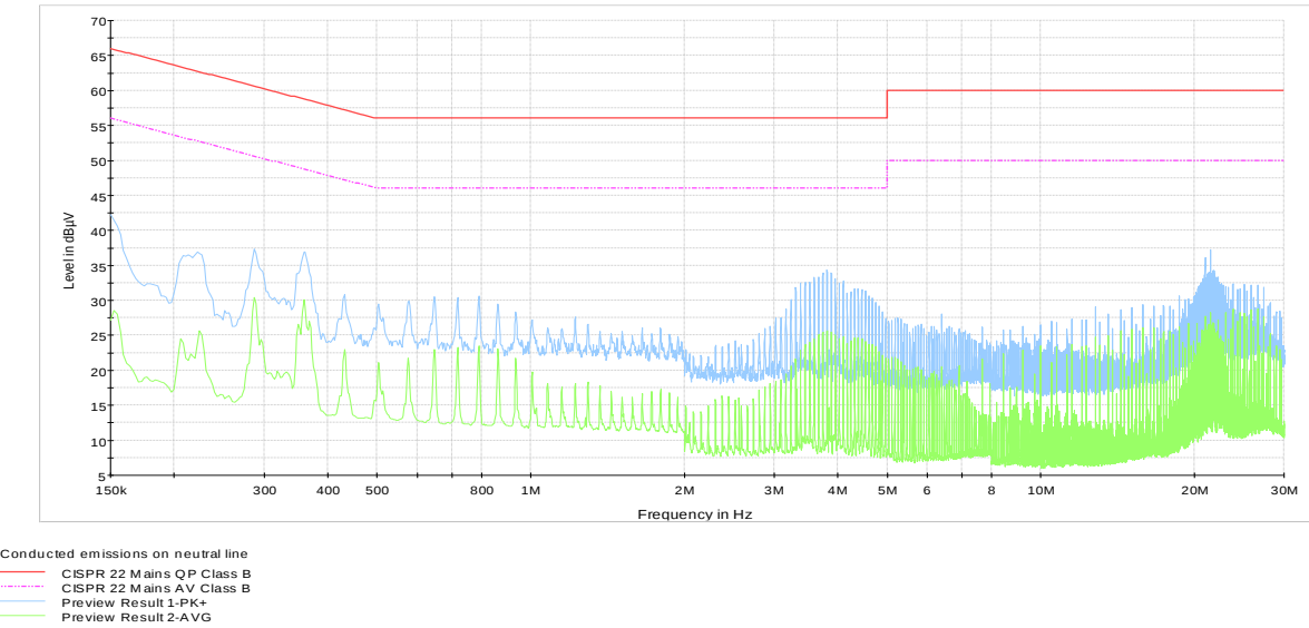
Plot 8.1-2: Conducted emissions on neutral line
