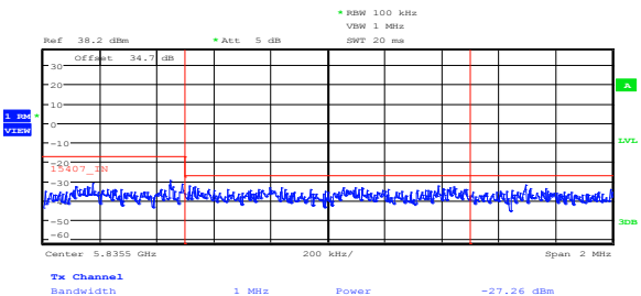
Figure 8.6-82: Upper IC band edge emission at 5.825 GHz, 802.11n HT40, ch1
