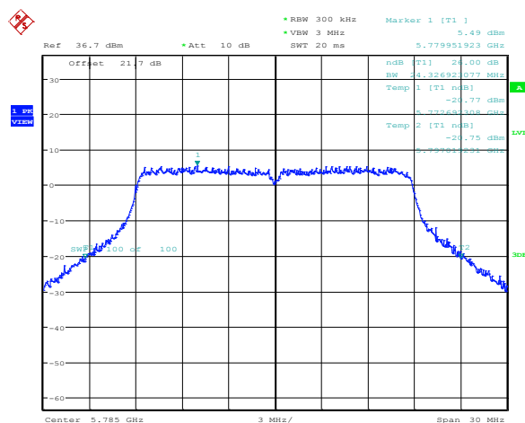
Figure 8.2-2: 26 dB bandwidth on 802.11n HT20, sample plot
