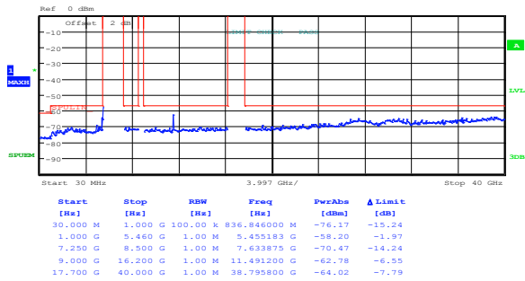
Figure 8.6-34: Peak spurious emissions within restricted bands at low channel, 802.11n HT20, ch1
