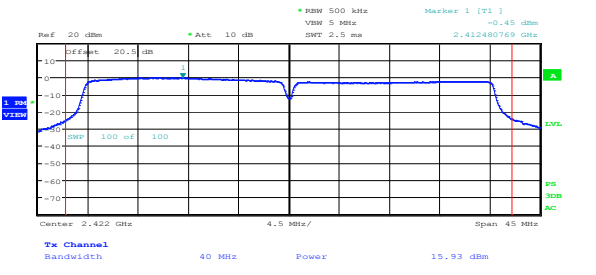
Figure 8.4-4: Output power on 802.11n HT40, sample plot
