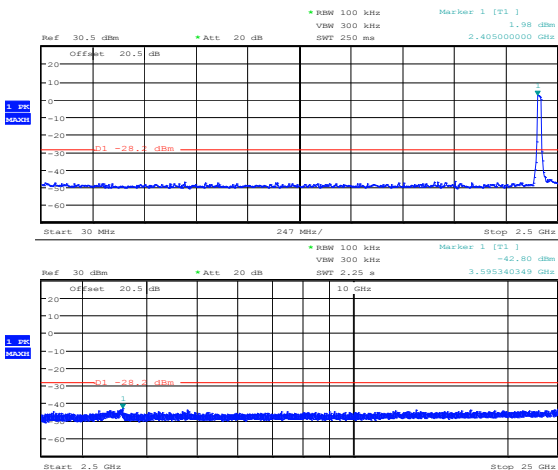
Figure 8.5-1: Conducted spurious emissions for 802.11b, cho, low channel
