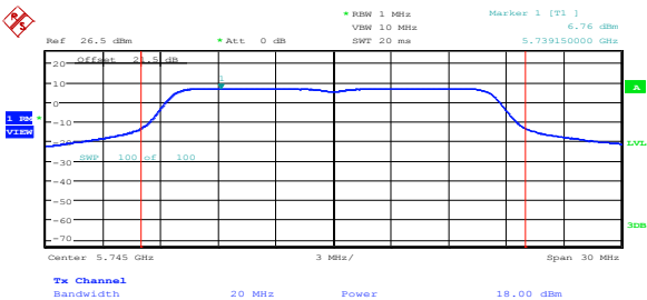
Figure 8.4-1: Output power on 802.11a, sample plot
