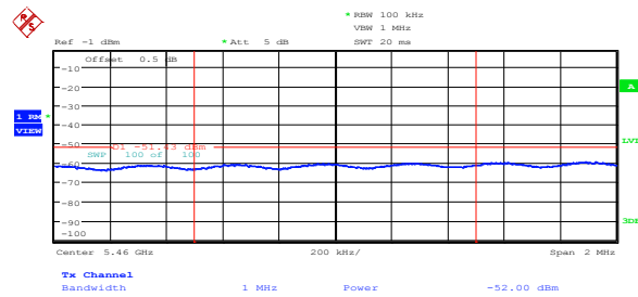
Figure 8.5-52: Average spurious emission at 5.46 GHz on IC low channel, 802.11n HT40, ch1
