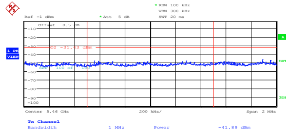
Figure 8.5-18: Peak spurious emission at 5.46 GHz on FCC low channel, 802.11n HT20, ch1
