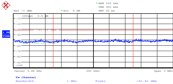
Figure 8.5-5: Peak spurious emission at 5.46 GHz on FCC high channel, 802.11n HT20, cho
