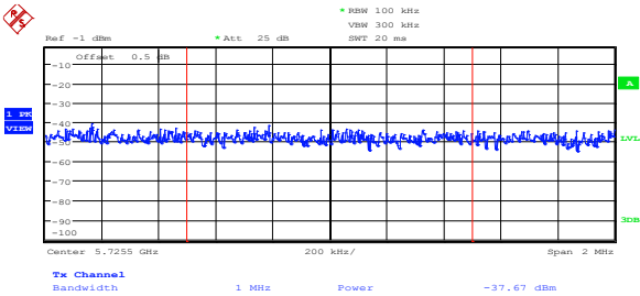
Figure 8.5-73: Upper band edge emission at 5.725 GHz on high channel, 802.11n HT40, cho (limit = -37.2 dBm/MHz)
