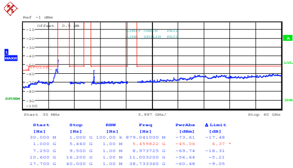
Figure 8.5-17: Peak spurious emissions within restricted bands at FCC low channel, 802.11n HT20, ch1
