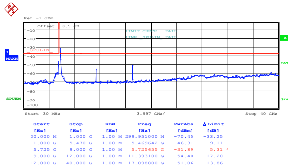
Figure 8.5-70: Spurious out-of-band emissions outside restricted bands at high channel, 802.11n HT20, cho
