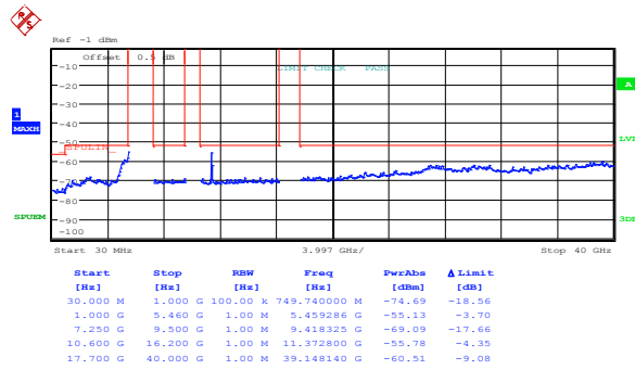
Figure 8.5-58: Peak spurious emissions within restricted bands at IC high channel, 802.11n HT40, ch1
