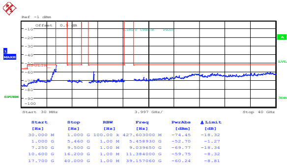
Figure 8.5-15: Peak spurious emissions within restricted bands at FCC high channel, 802.11n HT40, cho
