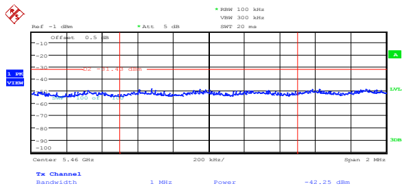
Figure 8.5-51: Peak spurious emission at 5.46 GHz on IC low channel, 802.11n HT40, ch1
