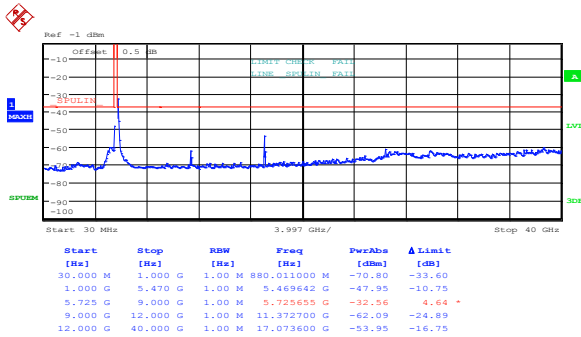
Figure 8.5-72: Spurious out-of-band emissions outside restricted bands at high channel, 802.11n HT40, cho
