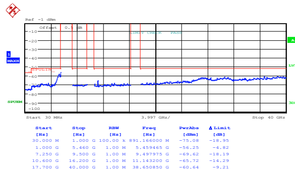
Figure 8.5-40: Peak spurious emissions within restricted bands at IC mid channel, 802.11n HT40, cho
