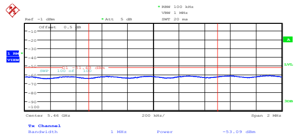
Figure 8.5-46: Average spurious emission at 5.46 GHz on IC low channel, 802.11a, ch1
