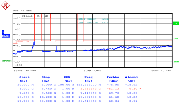
Figure 8.5-1: Peak spurious emissions within restricted bands at FCC low channel, 802.11a, cho
