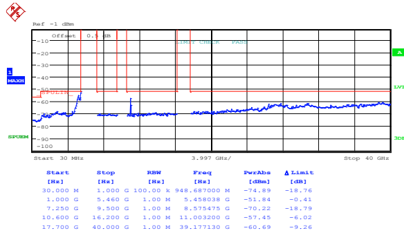
Figure 8.5-16: Peak spurious emissions within restricted bands at FCC low channel, 802.11a, ch1
