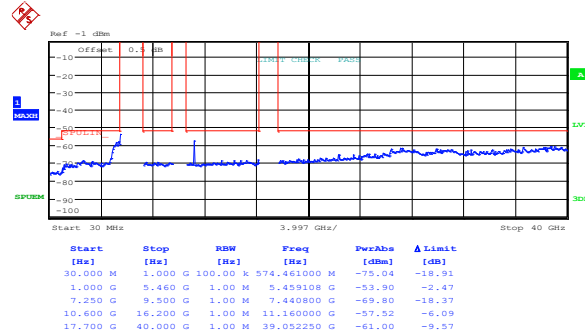
Figure 8.5-38: Peak spurious emissions within restricted bands at IC mid channel, 802.11a, cho
