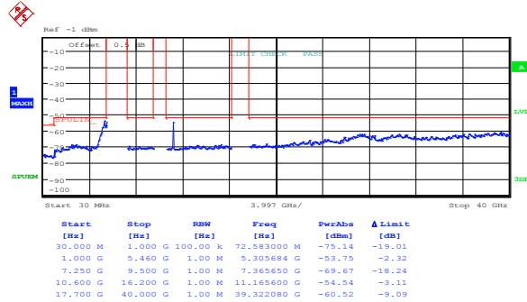
Figure 8.5-54: Peak spurious emissions within restricted bands at IC mid channel, 802.11n HT20, ch1
