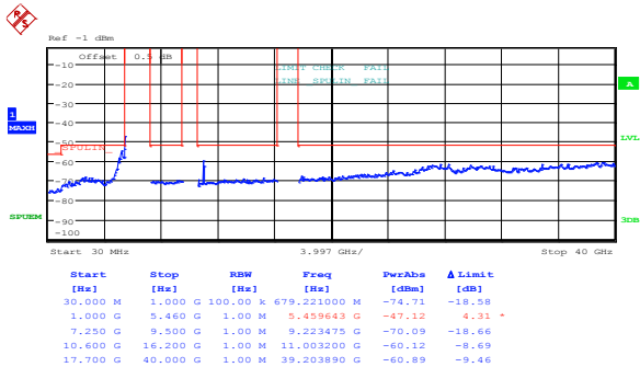
Figure 8.5-29: Peak spurious emissions within restricted bands at IC low channel, 802.11a, cho
