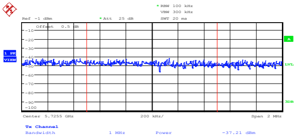
Figure 8.5-91: Upper band edge emission at 5.725 GHz on high channel, 802.11n HT40, ch1 (limit = -37.2 dBm/MHz)
