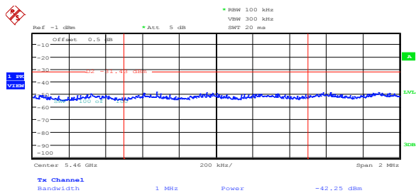
Figure 8.5-21: Peak spurious emission at 5.46 GHz on FCC low channel, 802.11n HT20, ch1
