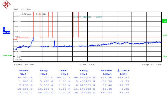
Figure 8.5-12: Peak spurious emissions within restricted bands at FCC mid channel, 802.11n HT40, cho
