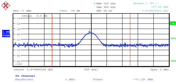
Figure 8.5-81: Spurious out-of-band emissions at 5.88 GHz on mid channel, 802.11a, ch1 (limit = -37.2 dBm/MHz)
