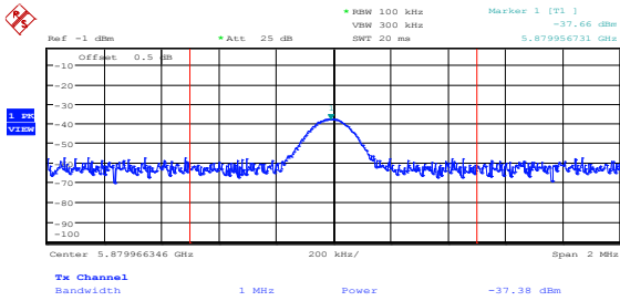
Figure 8.5-83: Spurious out-of-band emissions at 5.88 GHz on mid channel, 802.11n HT20, ch1 (limit = -37.2 dBm/MHz)
