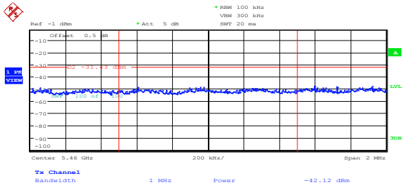
Figure 8.5-2: Peak spurious emission at 5.46 GHz on FCC high channel, 802.11a, cho
