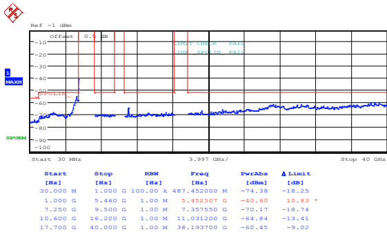
Figure 8.5-7: Peak spurious emissions within restricted bands at FCC low channel, 802.11n HT40, cho
