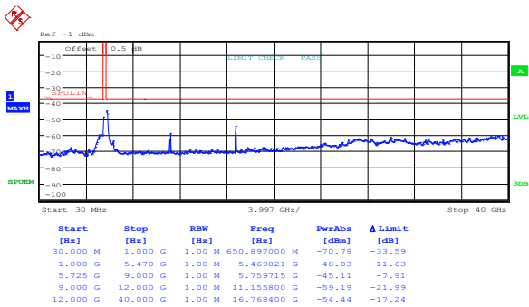
Figure 8.5-67: Spurious out-of-band emissions outside restricted bands at mid channel, 802.11n HT40, cho
