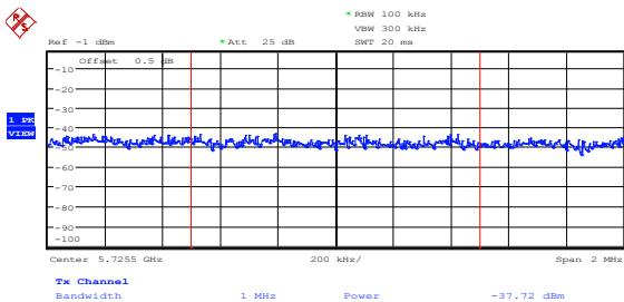
Figure 8.5-87: Upper band edge emission at 5.725 GHz on high channel, 802.11a, ch1 (limit = -37.2 dBm/MHz)
