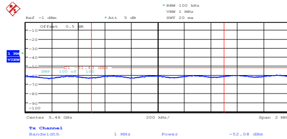
Figure 8.5-6: Average spurious emission at 5.46 GHz on FCC high channel, 802.11n HT20, cho
