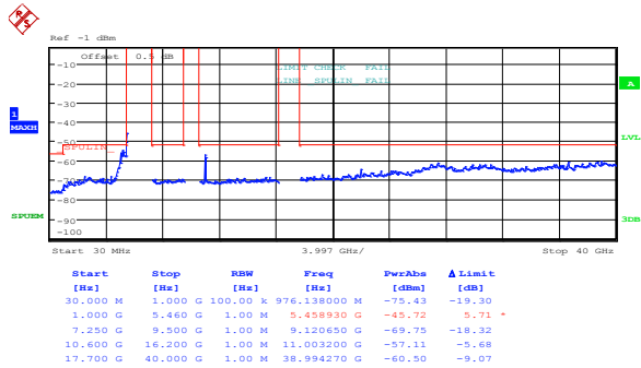
Figure 8.5-47: Peak spurious emissions within restricted bands at IC low channel, 802.11n HT20, ch1
