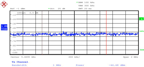
Figure 8.5-75: Lower band edge emission at 5.47 GHz on low channel, 802.11a, ch1 (limit = -37.2 dBm/MHz)
