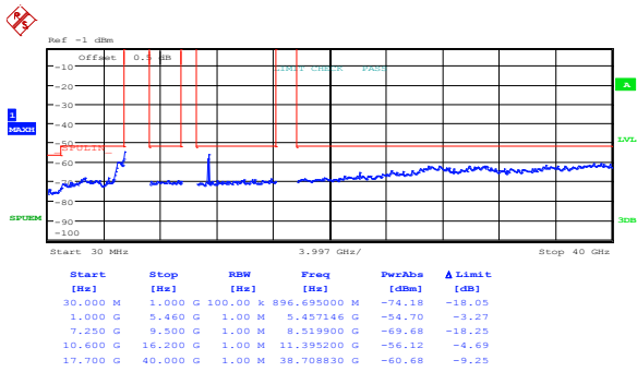
Figure 8.5-57: Peak spurious emissions within restricted bands at IC high channel, 802.11n HT20, ch1
