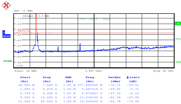
Figure 8.5-78: Spurious out-of-band emissions outside restricted bands at low channel, 802.11n HT40, ch1
