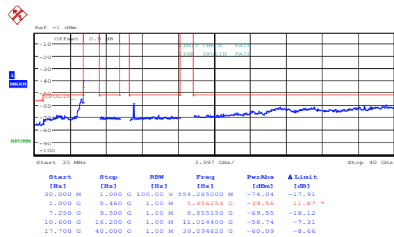
Figure 8.5-50: Peak spurious emissions within restricted bands at IC low channel, 802.11n HT40, ch1
