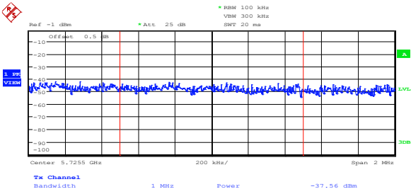
Figure 8.5-89: Upper band edge emission at 5.725 GHz on high channel, 802.11n HT20, ch1 (limit = -37.2 dBm/MHz)
