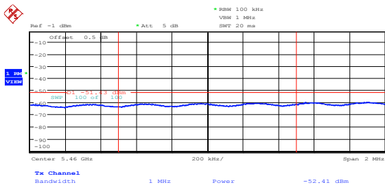
Figure 8.5-9: Average spurious emission at 5.46 GHz on FCC low channel, 802.11n HT40, cho
