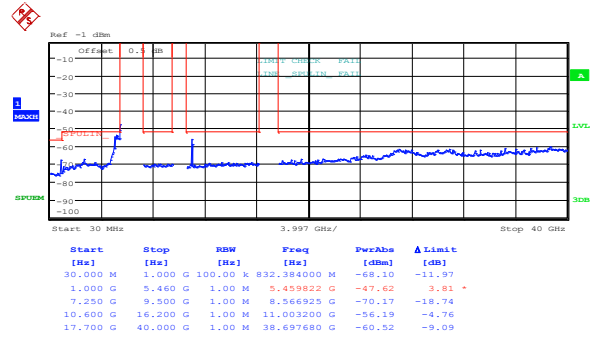
Figure 8.5-44: Peak spurious emissions within restricted bands at IC low channel, 802.11a, ch1
