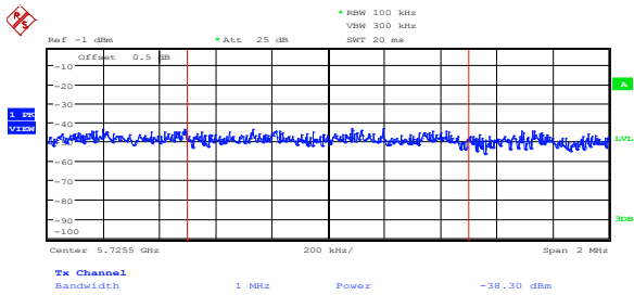
Figure 8.5-69: Upper band edge emission at 5.725 GHz on high channel, 802.11a, cho (limit = -37.2 dBm/MHz)
