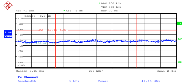
Figure 8.5-36: Peak spurious emission at 5.46 GHz on IC low channel, 802.11n HT40, cho
