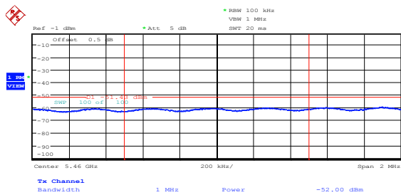
Figure 8.5-49: Average spurious emission at 5.46 GHz on IC low channel, 802.11n HT20, ch1
