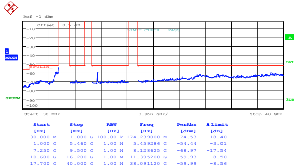
Figure 8.5-41: Peak spurious emissions within restricted bands at IC high channel, 802.11a, cho
