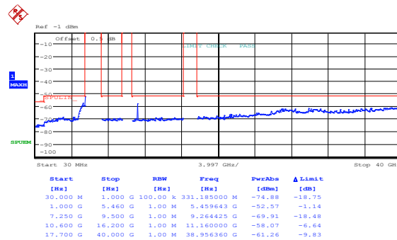
Figure 8.5-10: Peak spurious emissions within restricted bands at FCC mid channel, 802.11a, cho
