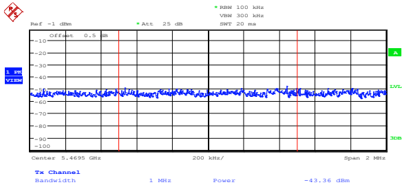
Figure 8.5-77: Lower band edge emission at 5.47 GHz on low channel, 802.11n HT20, ch1 (limit = -37.2 dBm/MHz)
