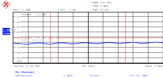
Figure 8.5-37: Average spurious emission at 5.46 GHz on IC low channel, 802.11n HT40, cho
