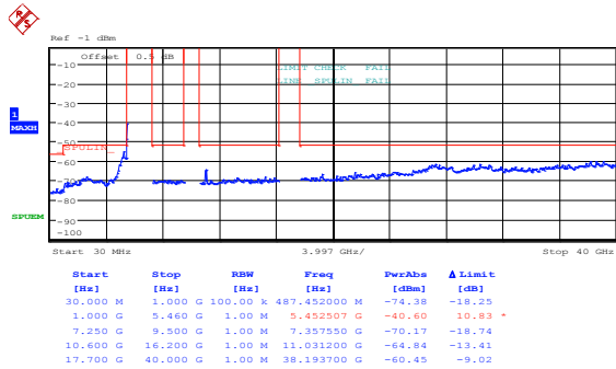
Figure 8.5-35: Peak spurious emissions within restricted bands at IC low channel, 802.11n HT40, cho
