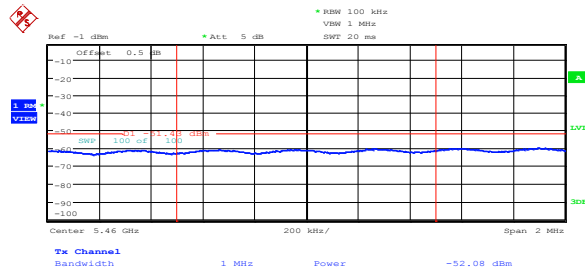
Figure 8.5-34: Average spurious emission at 5.46 GHz on IC low channel, 802.11n HT20, cho
