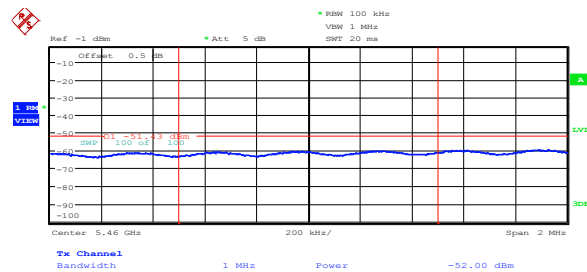
Figure 8.5-22: Average spurious emission at 5.46 GHz on FCC low channel, 802.11n HT20, ch1
