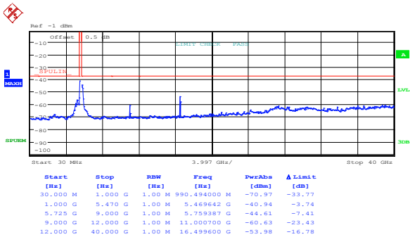
Figure 8.5-61: Spurious out-of-band emissions outside restricted bands at low channel, 802.11n HT20, cho
