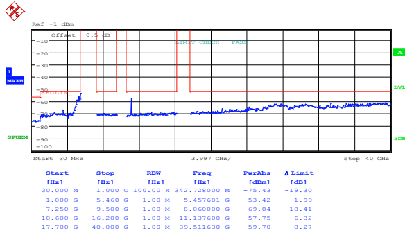
Figure 8.5-25: Peak spurious emissions within restricted bands at FCC mid channel, 802.11n HT40, ch1
