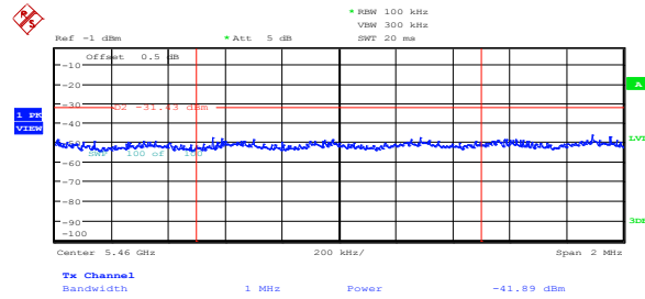
Figure 8.5-48: Peak spurious emission at 5.46 GHz on IC low channel, 802.11n HT20, ch1
