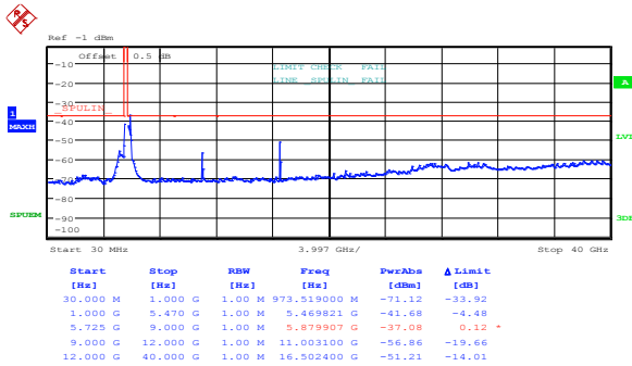
Figure 8.5-76: Spurious out-of-band emissions outside restricted bands at low channel, 802.11n HT20, ch1
