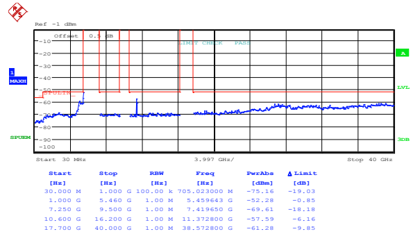
Figure 8.5-28: Peak spurious emissions within restricted bands at FCC high channel, 802.11n HT40, ch1
