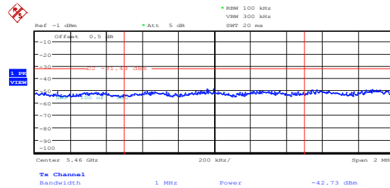
Figure 8.5-8: Peak spurious emission at 5.46 GHz on FCC low channel, 802.11n HT40, cho
