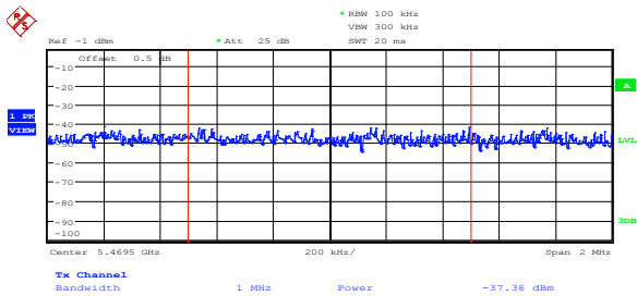
Figure 8.5-79: Lower band edge emission at 5.47 GHz on low channel, 802.11n HT40, ch1 (limit = -37.2 dBm/MHz)
