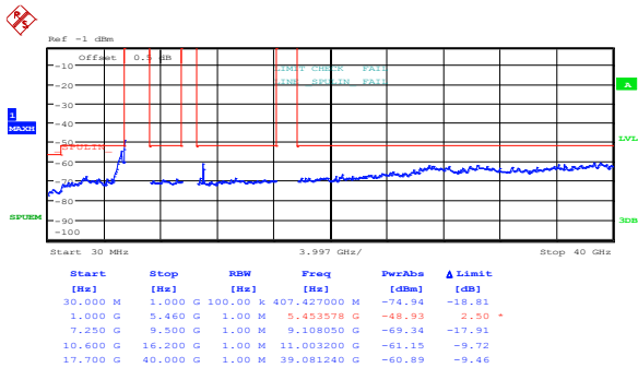
Figure 8.5-4: Peak spurious emissions within restricted bands at FCC low channel, 802.11n HT20, cho
