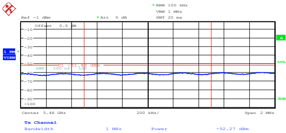
Figure 8.5-3: Average spurious emission at 5.46 GHz on FCC high channel, 802.11a, cho
