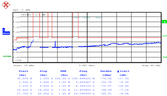
Figure 8.5-27: Peak spurious emissions within restricted bands at FCC high channel, 802.11n HT20, ch1
