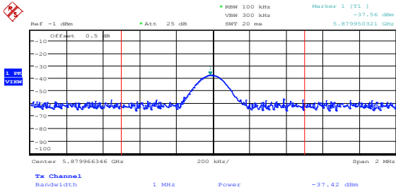
Figure 8.5-85: Spurious out-of-band emissions at 5.88 GHz on mid channel, 802.11n HT40, ch1 (limit = -37.2 dBm/MHz)
