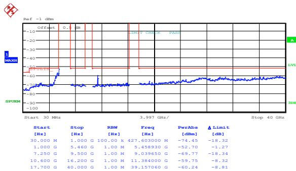
Figure 8.5-43: Peak spurious emissions within restricted bands at IC high channel, 802.11n HT40, cho
