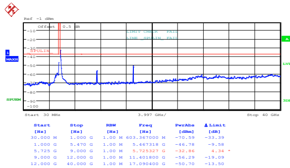
Figure 8.5-68: Spurious out-of-band emissions outside restricted bands at high channel, 802.11a, cho
