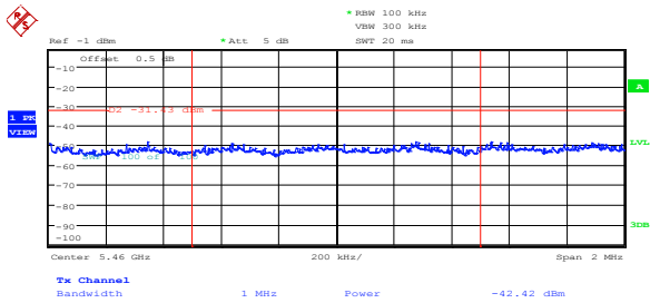
Figure 8.5-33: Peak spurious emission at 5.46 GHz on IC low channel, 802.11n HT20, cho
