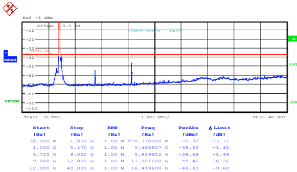
Figure 8.5-74: Spurious out-of-band emissions outside restricted bands at low channel, 802.11a, ch1
