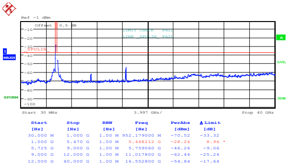
Figure 8.5-63: Spurious out-of-band emissions outside restricted bands at low channel, 802.11n HT40, cho
