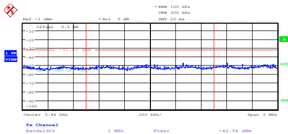
Figure 8.5-45: Peak spurious emission at 5.46 GHz on IC low channel, 802.11a, ch1
