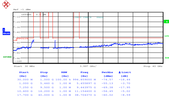
Figure 8.5-23: Peak spurious emissions within restricted bands at FCC mid channel, 802.11a, ch1
