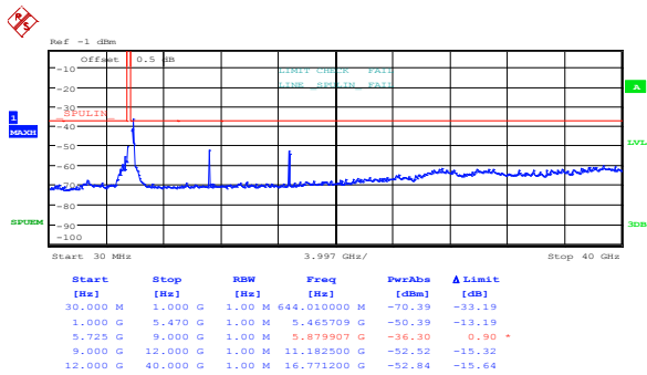
Figure 8.5-80: Spurious out-of-band emissions outside restricted bands at mid channel, 802.11a, ch1
