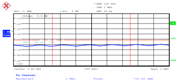
Figure 8.5-19: Average spurious emission at 5.46 GHz on FCC low channel, 802.11n HT20, ch1
