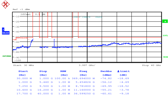
Figure 8.5-53: Peak spurious emissions within restricted bands at IC mid channel, 802.11a, ch1
