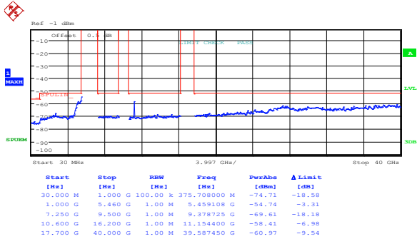
Figure 8.5-11: Peak spurious emissions within restricted bands at FCC mid channel, 802.11n HT20, cho
