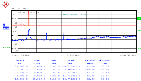
Figure 8.5-66: Spurious out-of-band emissions outside restricted bands at mid channel, 802.11n HT20, cho
