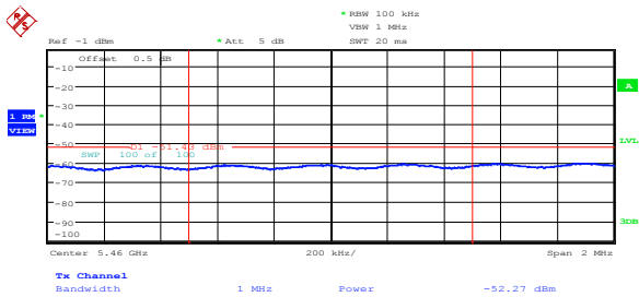
Figure 8.5-31: Average spurious emission at 5.46 GHz on IC low channel, 802.11a, cho
