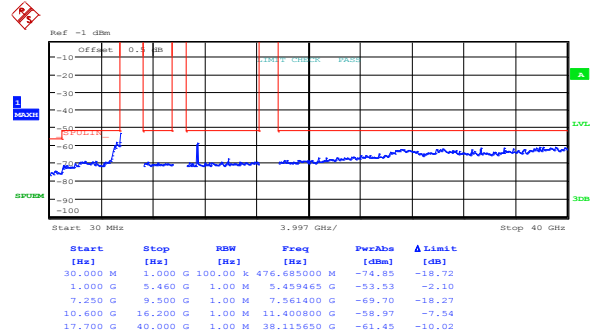
Figure 8.5-42: Peak spurious emissions within restricted bands at IC high channel, 802.11n HT20, cho
