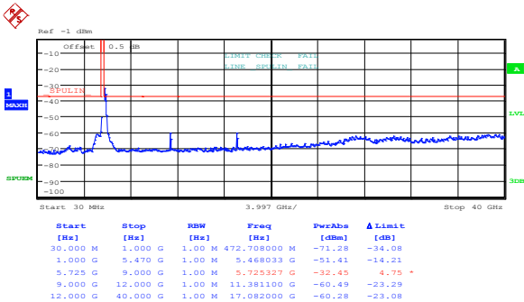
Figure 8.5-90: Spurious out-of-band emissions outside restricted bands at high channel, 802.11n HT40, ch1
