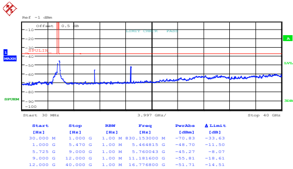
Figure 8.5-65: Spurious out-of-band emissions outside restricted bands at mid channel, 802.11a, cho
