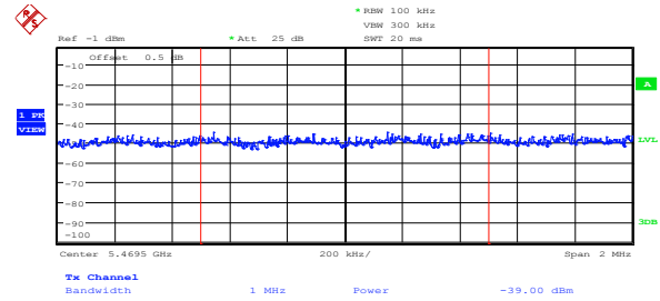
Figure 8.5-60: Lower band edge emission at 5.47 GHz on low channel, 802.11a, cho (limit = -37.2 dBm/MHz)
