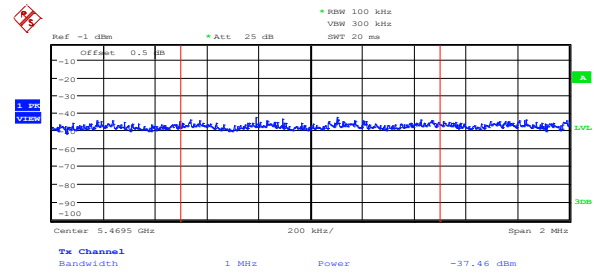
Figure 8.5-62: Lower band edge emission at 5.47 GHz on low channel, 802.11n HT20, cho (limit = -37.2 dBm/MHz)
