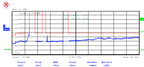
Figure 8.5-20: Peak spurious emissions within restricted bands at FCC low channel, 802.11n HT40, ch1
