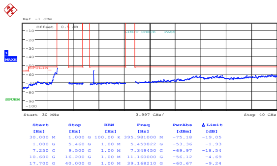
Figure 8.5-39: Peak spurious emissions within restricted bands at IC mid channel, 802.11n HT20, cho
