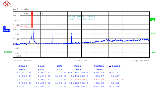
Figure 8.5-86: Spurious out-of-band emissions outside restricted bands at high channel, 802.11a, ch1
