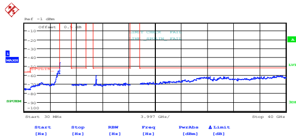
Figure 8.5-32: Peak spurious emissions within restricted bands at IC low channel, 802.11n HT20, cho
