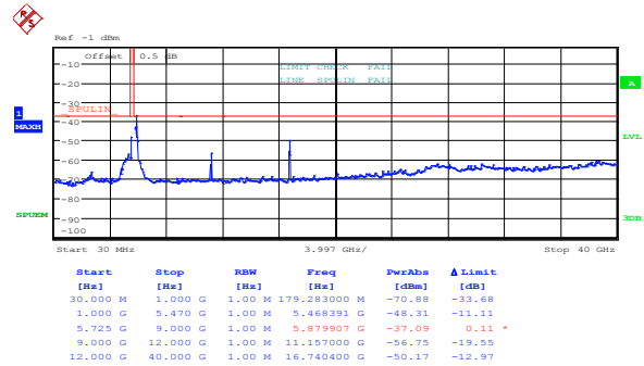
Figure 8.5-84: Spurious out-of-band emissions outside restricted bands at mid channel, 802.11n HT40, ch1
