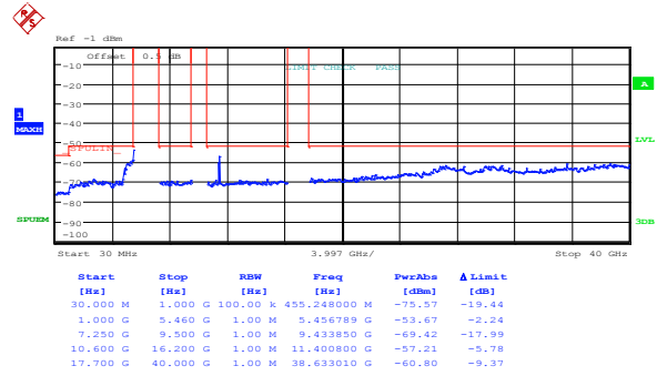
Figure 8.5-26: Peak spurious emissions within restricted bands at FCC high channel, 802.11a, ch1
