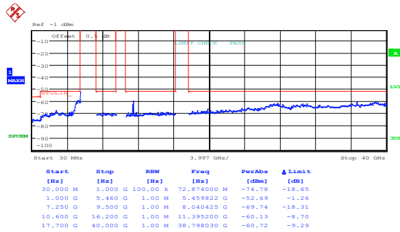
Figure 8.5-14: Peak spurious emissions within restricted bands at FCC high channel, 802.11n HT20, cho
