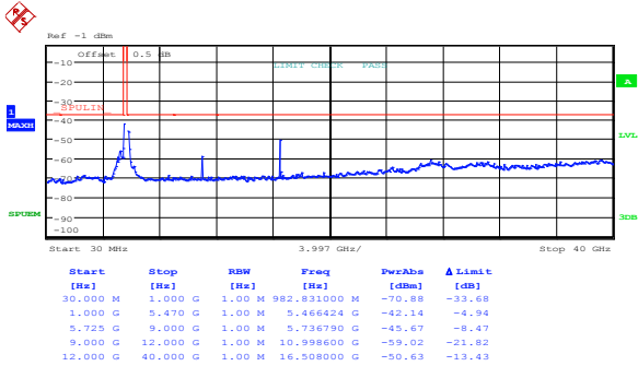
Figure 8.5-59: Spurious out-of-band emissions outside restricted bands at low channel, 802.11a, cho
