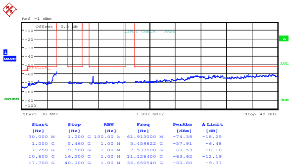
Figure 8.5-55: Peak spurious emissions within restricted bands at IC mid channel, 802.11n HT40, ch1
