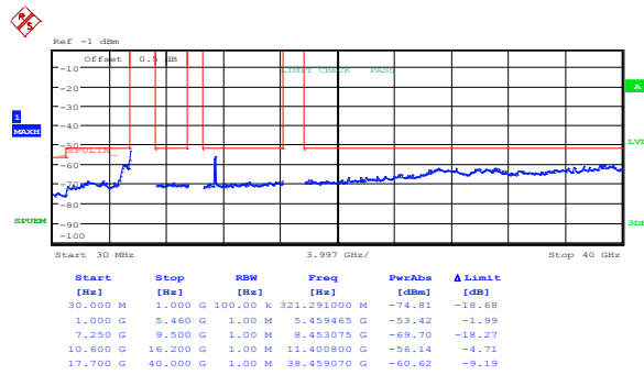
Figure 8.5-56: Peak spurious emissions within restricted bands at IC high channel, 802.11a, ch1
