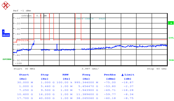
Figure 8.5-13: Peak spurious emissions within restricted bands at FCC high channel, 802.11a, cho
