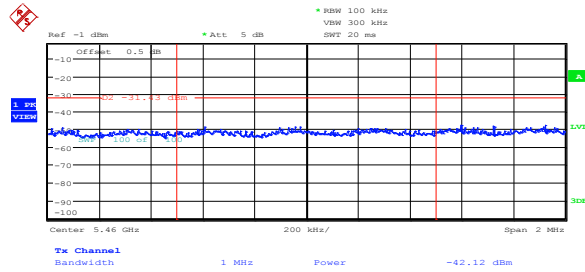
Figure 8.5-30: Peak spurious emission at 5.46 GHz on IC low channel, 802.11a, cho
