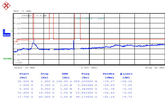
Figure 8.5-57: Peak spurious emissions within restricted bands at IC low channel, 802.11a, ch1
