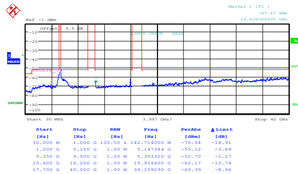
Figure 8.5-56: Peak spurious emissions within restricted bands at IC high channel, 802.11n HT40, cho
