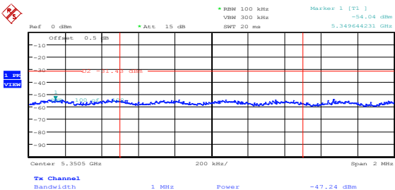
Figure 8.5-71: Peak spurious emission at 5.35 GHz on FCC high channel, 802.11n HT40, ch1
