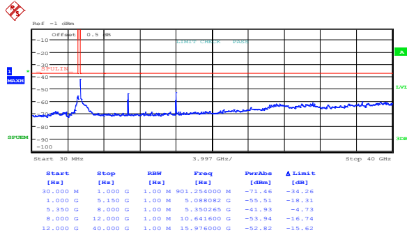
Figure 8.5-47: Spurious FCC out-of-band emissions outside restricted bands high channel, 802.11n HT20, ch1
