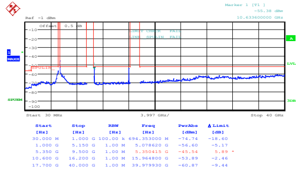
Figure 8.5-66: Peak spurious emissions within restricted bands at IC high channel, 802.11a, ch1
