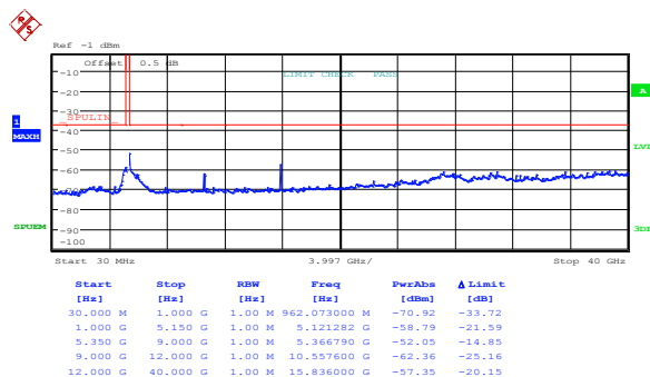
Figure 8.5-82: Spurious out-of-band emissions outside restricted bands at IC low channel, 802.11n HT20, ch1
