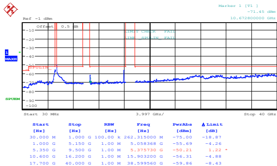
Figure 8.5-63: Peak spurious emissions within restricted bands at IC mid channel, 802.11n HT20, ch1
