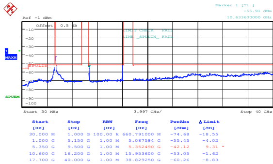
Figure 8.5-25: Peak spurious emissions within restricted bands at FCC high channel, 802.11n HT20, ch1
