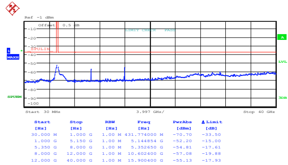
Figure 8.5-36: Spurious FCC out-of-band emissions outside restricted bands mid channel, 802.11a, cho
