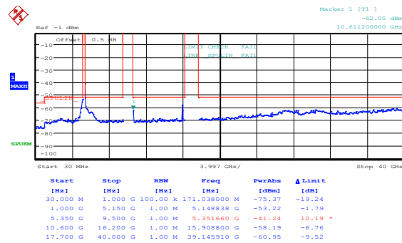
Figure 8.5-8: Peak spurious emissions within restricted bands at FCC high channel, 802.11n HT40, cho
