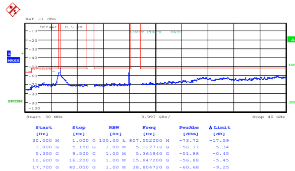
Figure 8.5-58: Peak spurious emissions within restricted bands at IC low channel, 802.11n HT20, ch1
