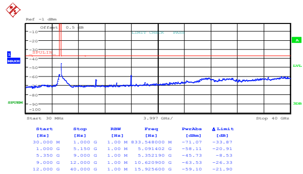
Figure 8.5-88: Spurious out-of-band emissions outside restricted bands at IC high channel, 802.11n HT40, ch1
