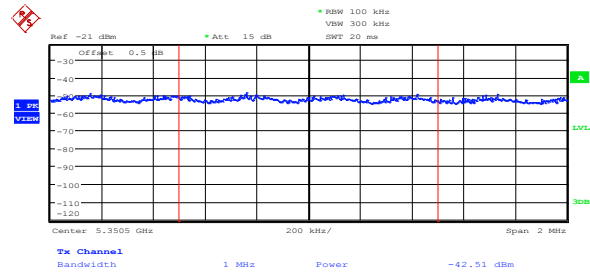
Figure 8.5-14: Peak spurious emission at 5.35 GHz on FCC high channel, 802.11n HT40, ch1
