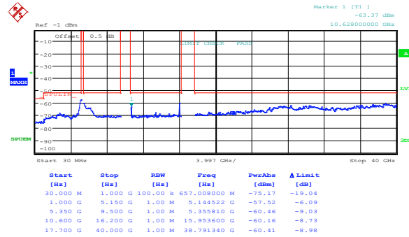
Figure 8.5-54: Peak spurious emissions within restricted bands at IC high channel, 802.11a, cho
