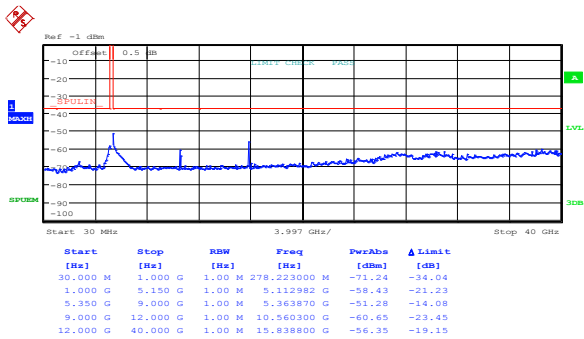
Figure 8.5-81: Spurious out-of-band emissions outside restricted bands at IC low channel, 802.11a, ch1
