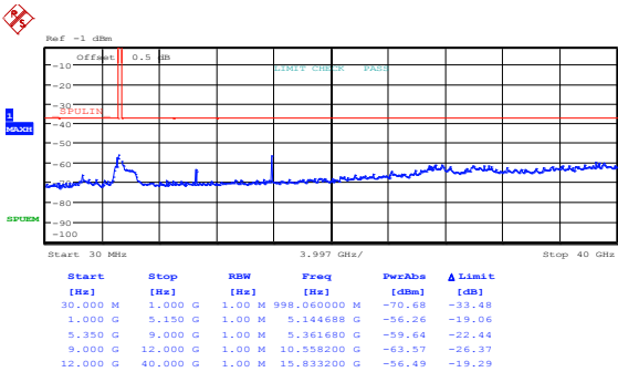
Figure 8.5-73: Spurious out-of-band emissions outside restricted bands at IC low channel, 802.11a, cho
