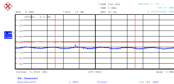
Figure 8.5-10: Average spurious emission at 5.35 GHz on FCC high channel, 802.11n HT40, cho
