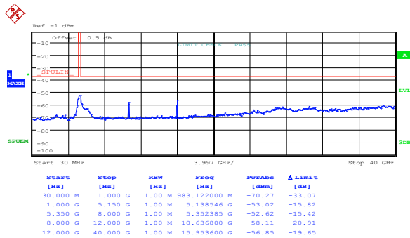
Figure 8.5-39: Spurious FCC out-of-band emissions outside restricted bands high channel, 802.11n HT20, cho
