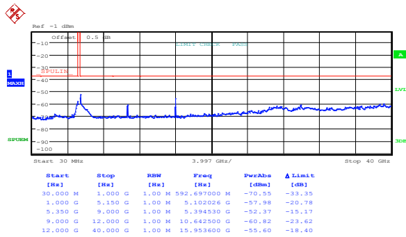
Figure 8.5-87: Spurious out-of-band emissions outside restricted bands at IC high channel, 802.11n HT20, ch1
