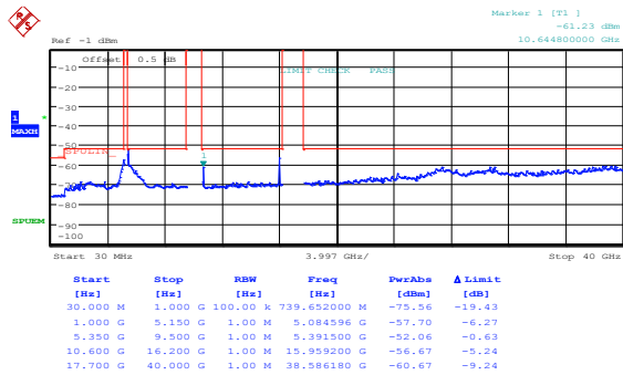
Figure 8.5-69: Peak spurious emissions within restricted bands at IC high channel, 802.11n HT20, ch1
