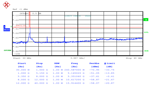
Figure 8.5-40: Spurious FCC out-of-band emissions outside restricted bands high channel, 802.11n HT40, cho
