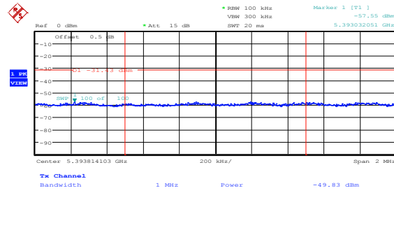
Figure 8.5-26: Peak spurious emission at 5.39 GHz on FCC high channel, 802.11n HT20, ch1
