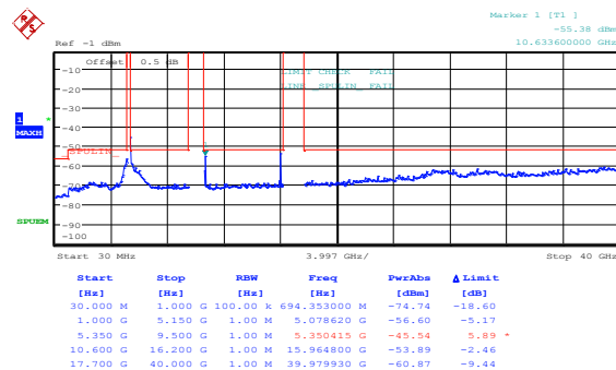
Figure 8.5-22: Peak spurious emissions within restricted bands at FCC high channel, 802.11a, ch1
