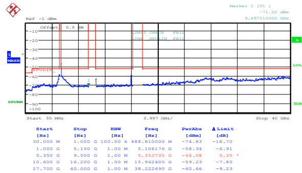
Figure 8.5-70: Peak spurious emissions within restricted bands at IC high channel, 802.11n HT40, ch1
