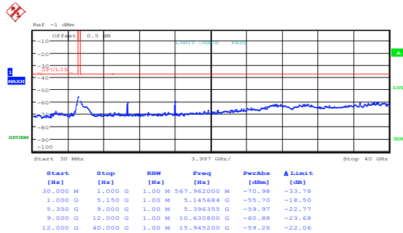
Figure 8.5-78: Spurious out-of-band emissions outside restricted bands at IC high channel, 802.11a, cho
