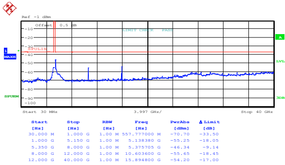
Figure 8.5-45: Spurious FCC out-of-band emissions outside restricted bands mid channel, 802.11n HT20, ch1
