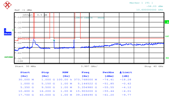
Figure 8.5-4: Peak spurious emissions within restricted bands at FCC mid channel, 802.11a, cho
