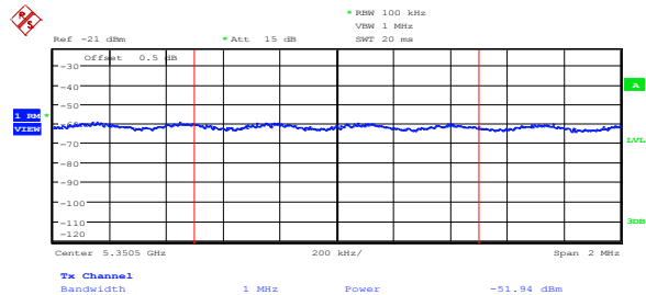
Figure 8.5-32: Average spurious emission at 5.35 GHz on FCC high channel, 802.11n HT40, ch1
