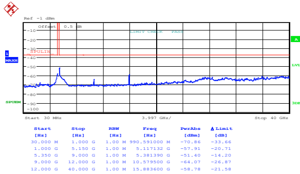
Figure 8.5-83: Spurious out-of-band emissions outside restricted bands at IC low channel, 802.11n HT40, ch1
