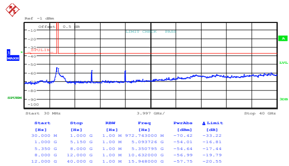
Figure 8.5-38: Spurious FCC out-of-band emissions outside restricted bands high channel, 802.11a, cho
