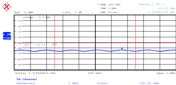
Figure 8.5-21: Average spurious emission at 5.37 GHz on FCC mid channel, 802.11n HT20, ch1
