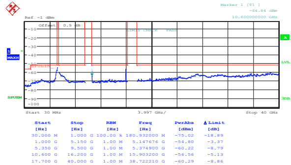
Figure 8.5-52: Peak spurious emissions within restricted bands at IC mid channel, 802.11a, cho
