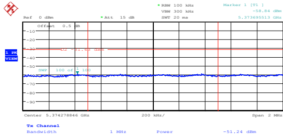
Figure 8.5-61: Peak spurious emission at 5.37 GHz on FCC mid channel, 802.11a, ch1
