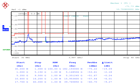
Figure 8.5-7: Peak spurious emissions within restricted bands at FCC high channel, 802.11n HT20, cho
