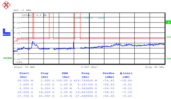
Figure 8.5-49: Peak spurious emissions within restricted bands at IC low channel, 802.11a, cho
