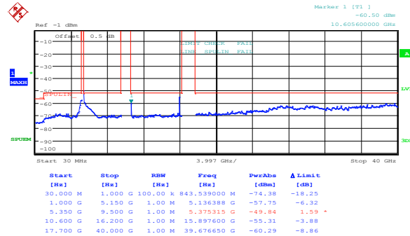
Figure 8.5-60: Peak spurious emissions within restricted bands at IC mid channel, 802.11a, ch1
