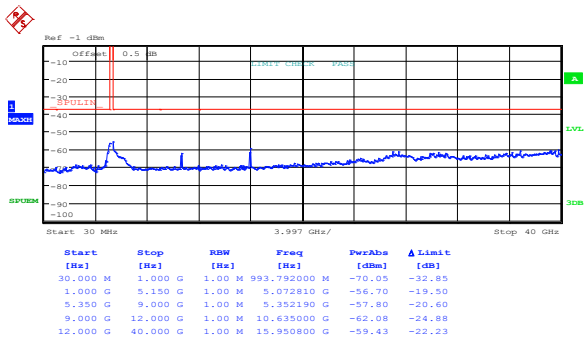
Figure 8.5-79: Spurious out-of-band emissions outside restricted bands at IC high channel, 802.11n HT20, cho
