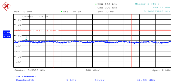
Figure 8.5-9: Peak spurious emission at 5.35 GHz on FCC high channel, 802.11n HT40, cho
