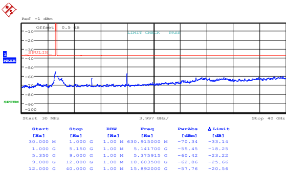
Figure 8.5-76: Spurious out-of-band emissions outside restricted bands at IC mid channel, 802.11a, cho
