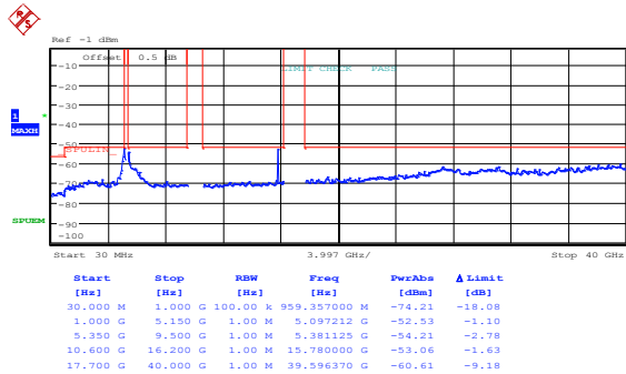
Figure 8.5-11: Peak spurious emissions within restricted bands at FCC low channel, 802.11a, ch1
