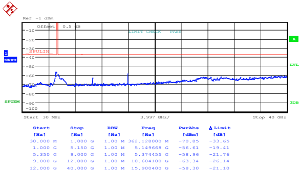
Figure 8.5-77: Spurious out-of-band emissions outside restricted bands at IC mid channel, 802.11n HT20, cho
