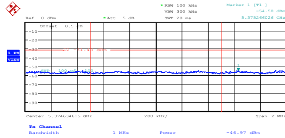
Figure 8.5-20: Peak spurious emission at 5.37 GHz on FCC mid channel, 802.11n HT20, ch1
