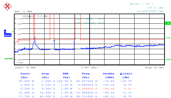
Figure 8.5-16: Peak spurious emissions within restricted bands at FCC mid channel, 802.11a, ch1
