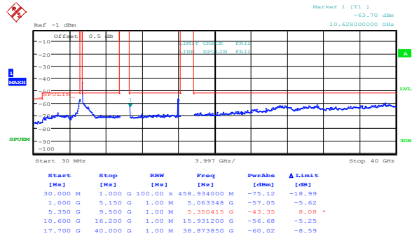
Figure 8.5-30: Peak spurious emissions within restricted bands at FCC high channel, 802.11n HT40, ch1
