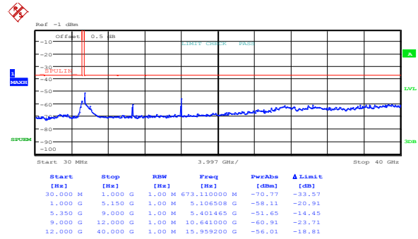
Figure 8.5-86: Spurious out-of-band emissions outside restricted bands at IC high channel, 802.11a, ch1
