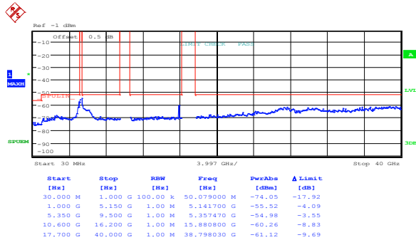
Figure 8.5-51: Peak spurious emissions within restricted bands at IC low channel, 802.11n HT40, cho
