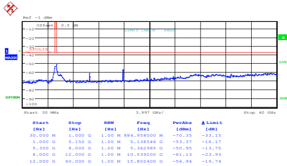
Figure 8.5-35: Spurious FCC out-of-band emissions outside restricted bands low channel, 802.11n HT40, cho
