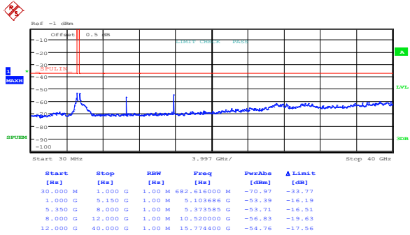
Figure 8.5-42: Spurious FCC out-of-band emissions outside restricted bands low channel, 802.11n HT20, ch1
