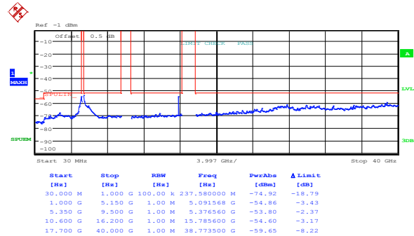
Figure 8.5-12: Peak spurious emissions within restricted bands at FCC low channel, 802.11n HT20, ch1
