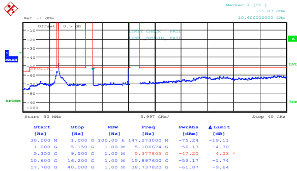
Figure 8.5-19: Peak spurious emissions within restricted bands at FCC mid channel, 802.11n HT20, ch1
