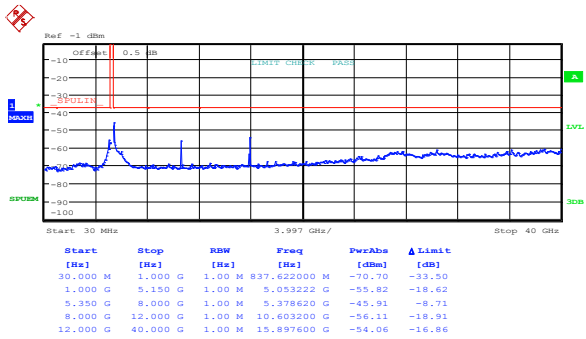
Figure 8.5-44: Spurious FCC out-of-band emissions outside restricted bands mid channel, 802.11a, ch1
