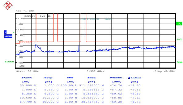
Figure 8.5-50: Peak spurious emissions within restricted bands at IC low channel, 802.11n HT20, cho
