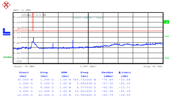
Figure 8.5-85: Spurious out-of-band emissions outside restricted bands at IC mid channel, 802.11n HT20, ch1
