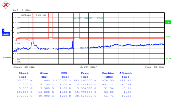
Figure 8.5-3: Peak spurious emissions within restricted bands at FCC low channel, 802.11n HT40, cho
