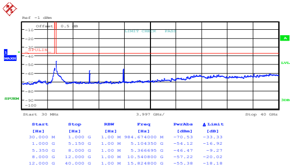
Figure 8.5-43: Spurious FCC out-of-band emissions outside restricted bands low channel, 802.11n HT40, ch1
