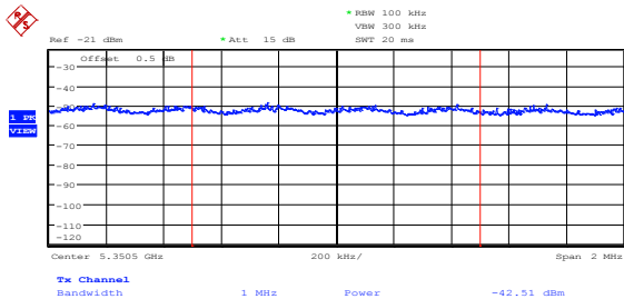
Figure 8.5-31: Peak spurious emission at 5.35 GHz on FCC high channel, 802.11n HT40, ch1
