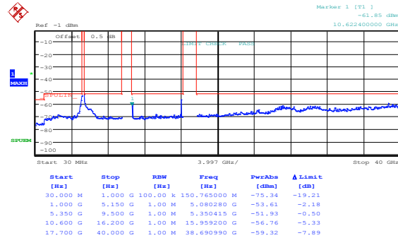
Figure 8.5-6: Peak spurious emissions within restricted bands at FCC high channel, 802.11a, cho
