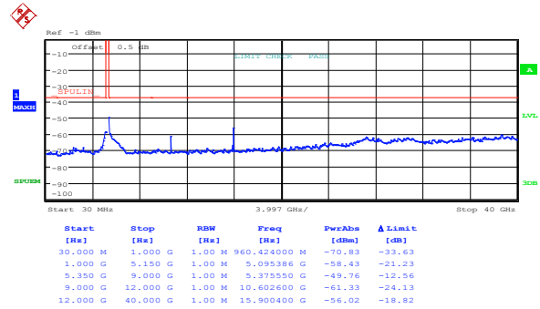
Figure 8.5-84: Spurious out-of-band emissions outside restricted bands at IC mid channel, 802.11a, ch1
