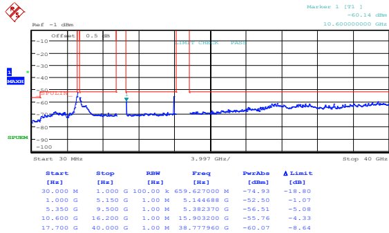
Figure 8.5-5: Peak spurious emissions within restricted bands at FCC mid channel, 802.11n HT20, cho
