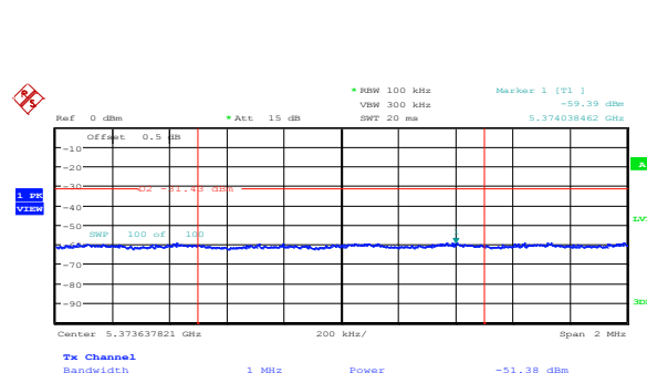
Figure 8.5-64: Peak spurious emission at 5.37 GHz on FCC mid channel, 802.11n HT20, ch1
