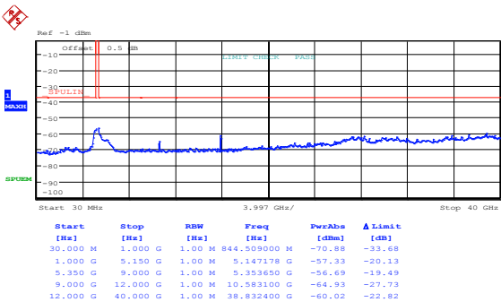
Figure 8.5-75: Spurious out-of-band emissions outside restricted bands at IC low channel, 802.11n HT40, cho
