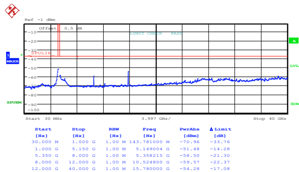
Figure 8.5-34: Spurious FCC out-of-band emissions outside restricted bands low channel, 802.11n HT20, cho
