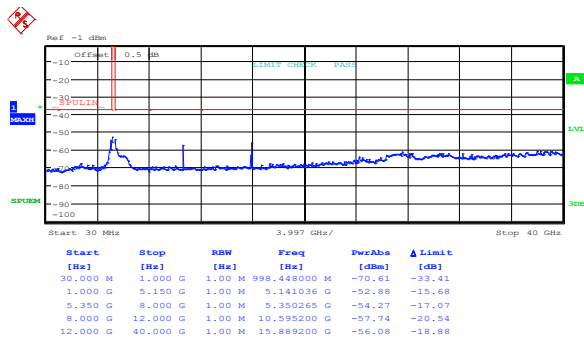
Figure 8.5-37: Spurious FCC out-of-band emissions outside restricted bands mid channel, 802.11n HT20, cho
