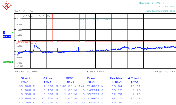
Figure 8.5-59: Peak spurious emissions within restricted bands at IC low channel, 802.11n HT40, ch1
