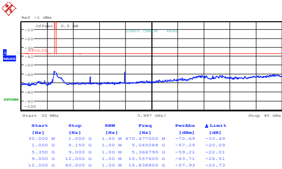
Figure 8.5-74: Spurious out-of-band emissions outside restricted bands at IC low channel, 802.11n HT20, cho
