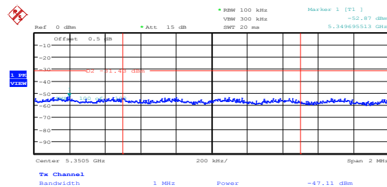
Figure 8.5-28: Peak spurious emission at 5.35 GHz on FCC high channel, 802.11n HT20, ch1
