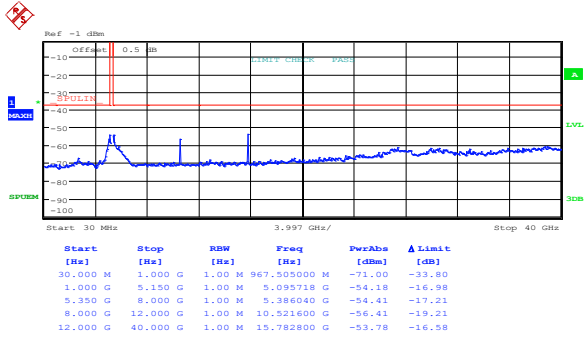
Figure 8.5-41: Spurious FCC out-of-band emissions outside restricted bands low channel, 802.11a, ch1
