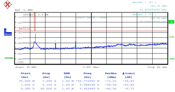
Figure 8.5-48: Spurious FCC out-of-band emissions outside restricted bands high channel, 802.11n HT40, ch1
