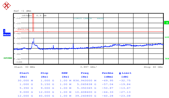
Figure 8.5-80: Spurious out-of-band emissions outside restricted bands at IC high channel, 802.11n HT40, cho
