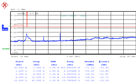
Figure 8.5-33: Spurious FCC out-of-band emissions outside restricted bands low channel, 802.11a, cho
