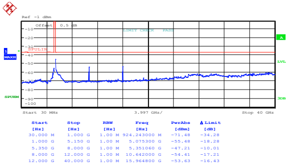
Figure 8.5-46: Spurious FCC out-of-band emissions outside restricted bands high channel, 802.11a, ch1
