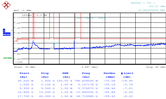
Figure 8.5-53: Peak spurious emissions within restricted bands at IC mid channel, 802.11n HT20, cho
