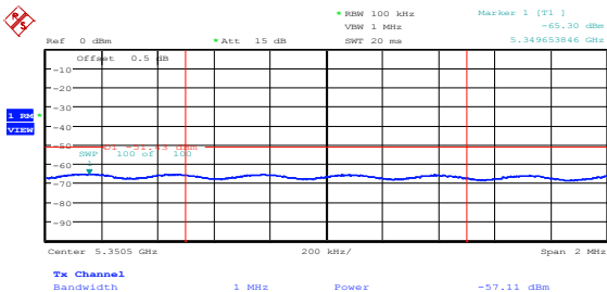
Figure 8.5-72: Average spurious emission at 5.35 GHz on FCC high channel, 802.11n HT40, ch1
