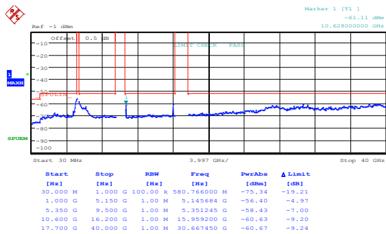
Figure 8.5-55: Peak spurious emissions within restricted bands at IC high channel, 802.11n HT20, cho
