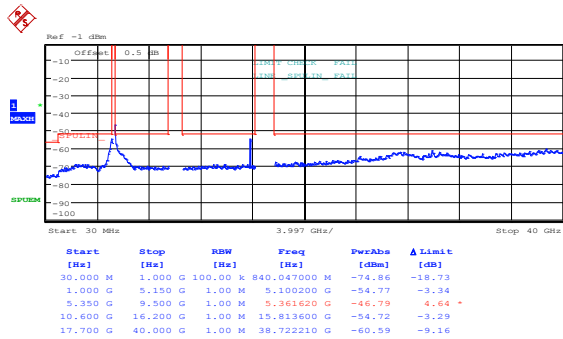
Figure 8.5-13: Peak spurious emissions within restricted bands at FCC low channel, 802.11n HT40, ch1
