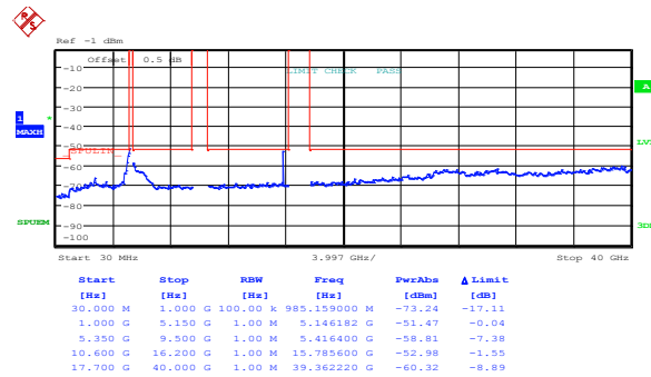
Figure 8.5-2: Peak spurious emissions within restricted bands at FCC low channel, 802.11n HT20, cho
