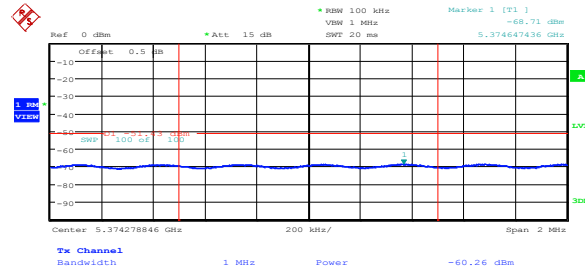
Figure 8.5-62: Average spurious emission at 5.37 GHz on FCC mid channel, 802.11a, ch1
