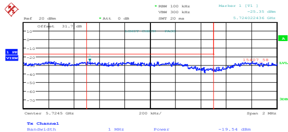
Figure 8.5-20: Lower band edge emissions at 5725 MHz, 802.11a, high channel, ch1
