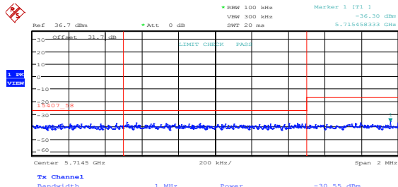
Figure 8.5-35: Lower band edge emissions at 5715 MHz, 802.11n HT20, low channel, ch1
