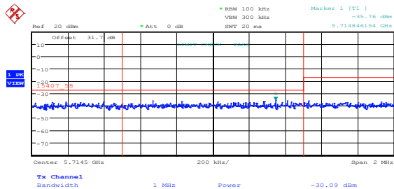
Figure 8.5-19: Lower band edge emissions at 5715 MHz, 802.11a, high channel, ch1
