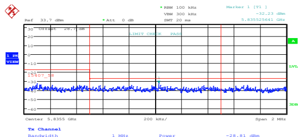
Figure 8.5-22: Upper band edge emissions at 5835 MHz, 802.11a, high channel, ch1
