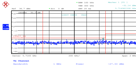
Figure 8.5-56: Lower band edge emissions at 5715 MHz, 802.11n HT40, low channel, ch1
