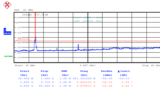
Figure 8.5-44: Conducted spurious emissions outside restricted bands, 802.11n HT20, high channel, ch1
