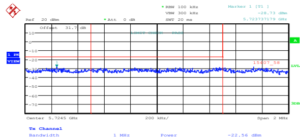
Figure 8.5-62: Lower band edge emissions at 5725 MHz, 802.11n HT40, high channel, ch1
