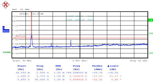
Figure 8.5-13: Conducted spurious emissions outside restricted bands, 802.11a, mid channel, ch1
