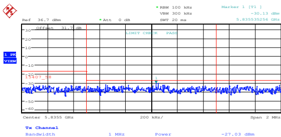
Figure 8.5-33: Upper band edge emissions at 5835 MHz, 802.11n HT20, high channel, cho
