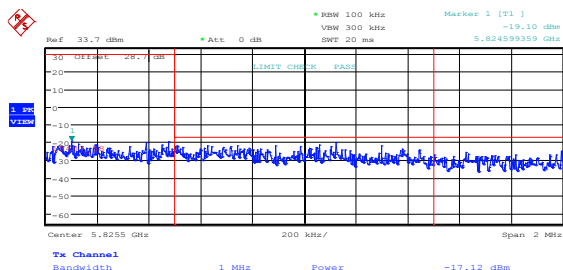
Figure 8.5-21: Upper band edge emissions at 5825 MHz, 802.11a, high channel, ch1
