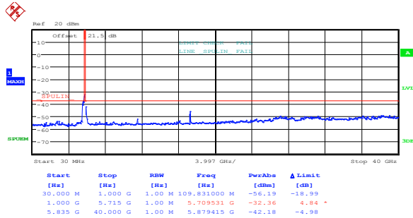
Figure 8.5-23: Conducted spurious emissions outside restricted bands, 802.11n HT20, low channel, cho
