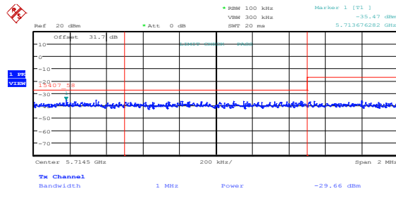
Figure 8.5-40: Lower band edge emissions at 5715 MHz, 802.11n HT20, mid channel, ch1
