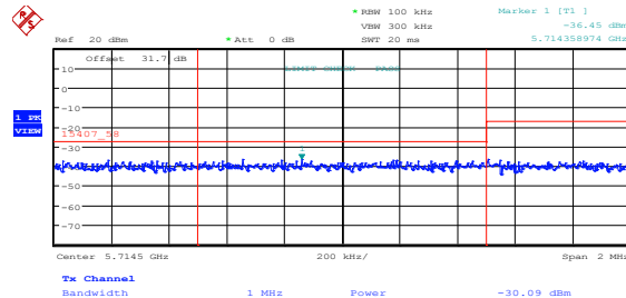
Figure 8.5-14: Lower band edge emissions at 5715 MHz, 802.11a, mid channel, ch1
