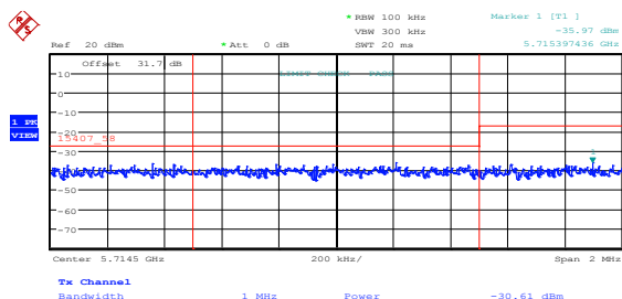
Figure 8.5-45: Lower band edge emissions at 5715 MHz, 802.11n HT20, high channel, ch1
