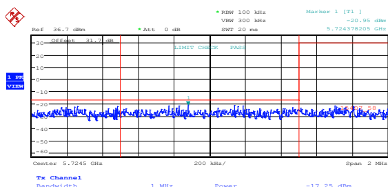
Figure 8.5-57: Lower band edge emissions at 5725 MHz, 802.11n HT40, low channel, ch1
