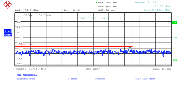
Figure 8.5-24: Lower band edge emissions at 5715 MHz, 802.11n HT20, low channel, cho
