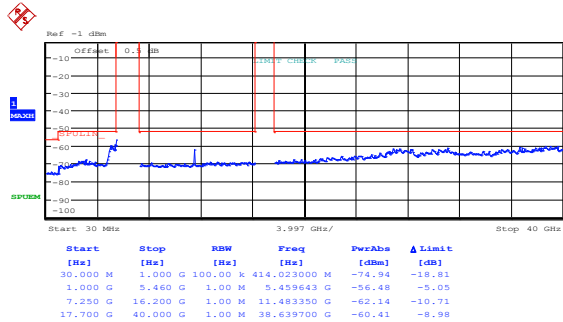
Figure 8.5-81: Conducted peak spurious emissions within restricted bands, 802.11n HT20, low channel, ch1
