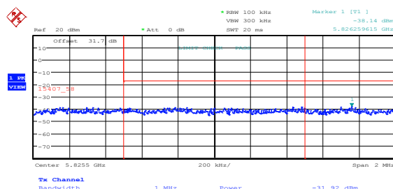
Figure 8.5-58: Upper band edge emissions at 5825 MHz, 802.11n HT40, low channel, ch1
