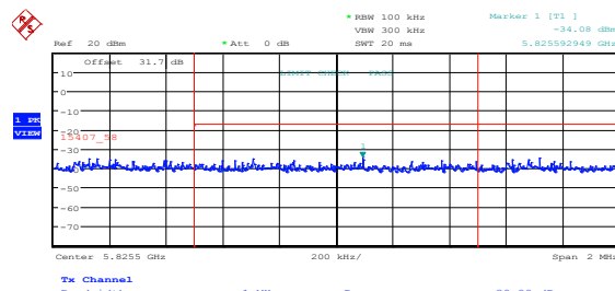
Figure 8.5-16: Upper band edge emissions at 5825 MHz, 802.11a, mid channel, ch1
