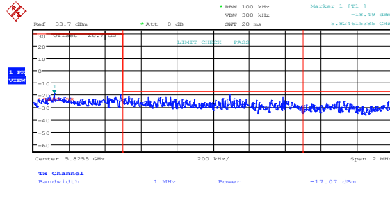
Figure 8.5-32: Upper band edge emissions at 5825 MHz, 802.11n HT20, high channel, cho
