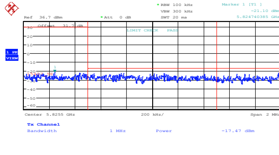
Figure 8.5-8: Upper band edge emissions at 5825 MHz, 802.11a, high channel, cho
