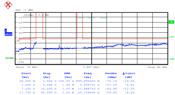
Figure 8.5-70: Conducted peak spurious emissions within restricted bands, 802.11a, low channel, ch1
