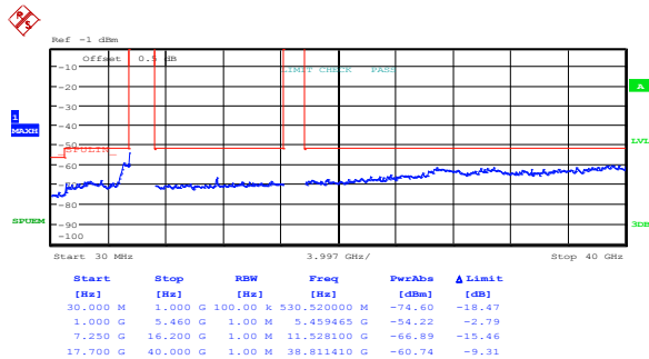
Figure 8.5-85: Conducted peak spurious emissions within restricted bands, 802.11n HT40, low channel, cho
