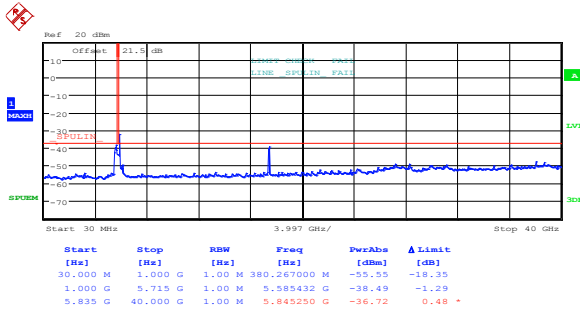
Figure 8.5-31: Conducted spurious emissions outside restricted bands, 802.11n HT20, high channel, cho
