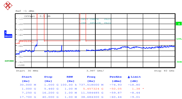
Figure 8.5-86: Conducted peak spurious emissions within restricted bands, 802.11n HT40, high channel, cho
