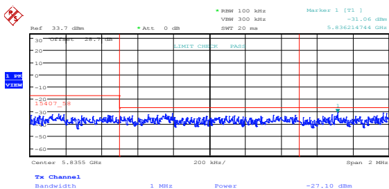
Figure 8.5-9: Upper band edge emissions at 5835 MHz, 802.11a, high channel, cho
