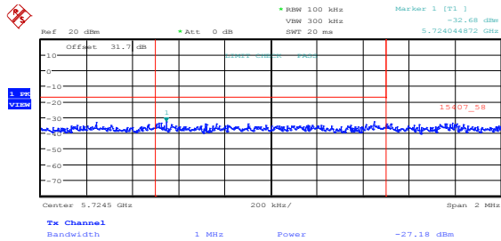
Figure 8.5-41: Lower band edge emissions at 5725 MHz, 802.11n HT20, mid channel, ch1
