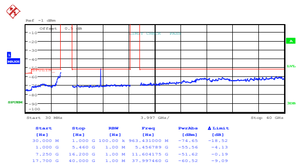
Figure 8.5-82: Conducted peak spurious emissions within restricted bands, 802.11n HT20, mid channel, ch1
