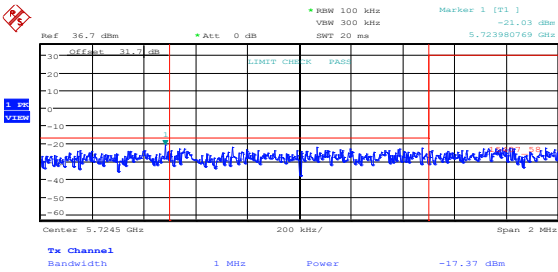
Figure 8.5-3: Lower band edge emissions at 5725 MHz, 802.11a, low channel, cho
