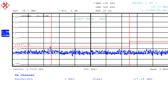
Figure 8.5-2: Lower band edge emissions at 5715 MHz, 802.11a, low channel, cho
