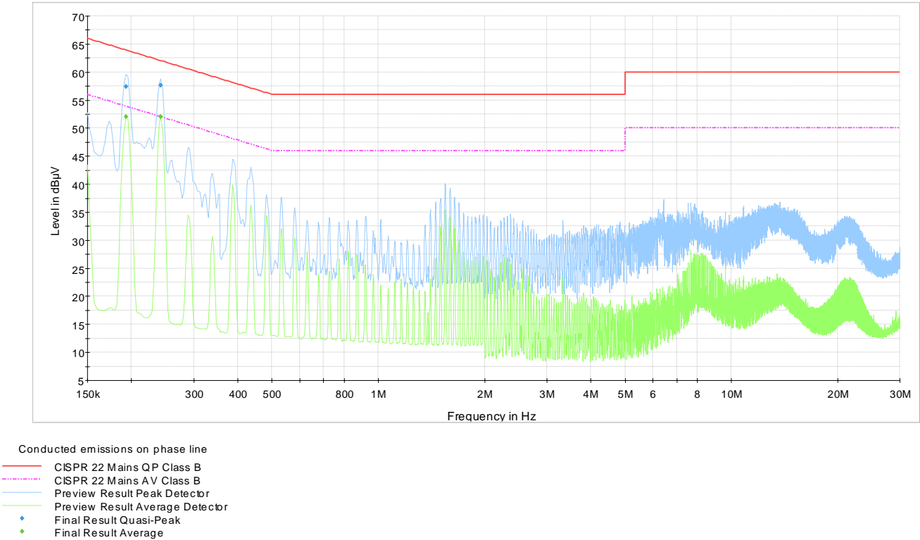
Plot 8.1-1: Conducted emissions on phase line
