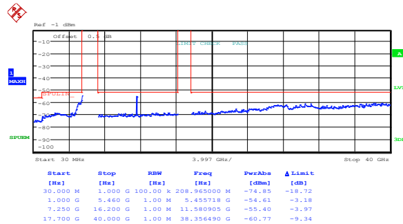
Figure 8.5-89: Conducted peak spurious emissions within restricted bands, 802.11n HT420, high channel, ch1
