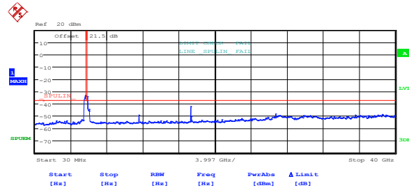
Figure 8.5-26: Conducted spurious emissions outside restricted bands, 802.11n HT20, mid channel, cho
