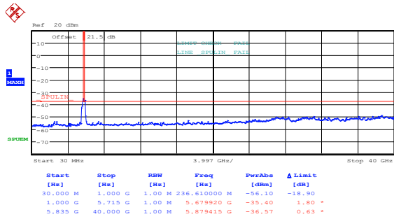
Figure 8.5-55: Conducted spurious emissions outside restricted bands, 802.11n HT40, low channel, ch1
