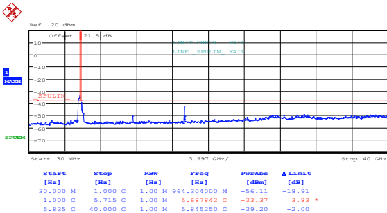
Figure 8.5-4: Conducted spurious emissions outside restricted bands, 802.11a, mid channel, cho
