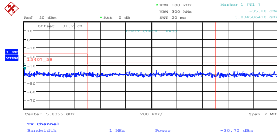
Figure 8.5-30: Upper band edge emissions at 5835 MHz, 802.11n HT20, mid channel, cho
