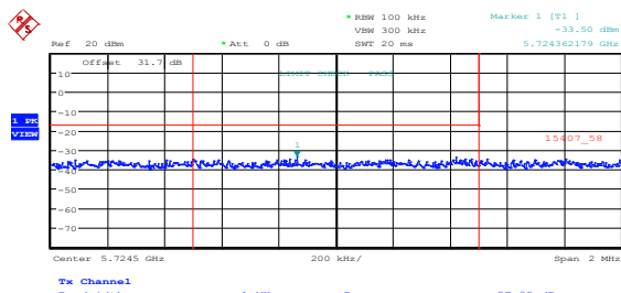
Figure 8.5-15: Lower band edge emissions at 5725 MHz, 802.11a, mid channel, ch1
