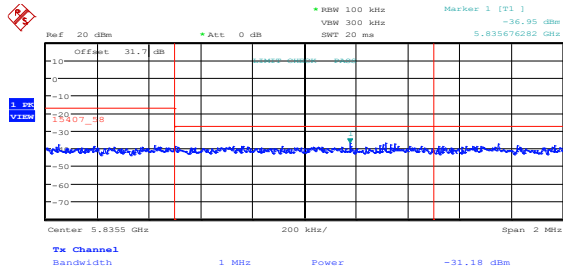
Figure 8.5-43: Upper band edge emissions at 5835 MHz, 802.11n HT20, mid channel, ch1
