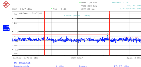
Figure 8.5-12: Lower band edge emissions at 5725 MHz, 802.11a, low channel, ch1
