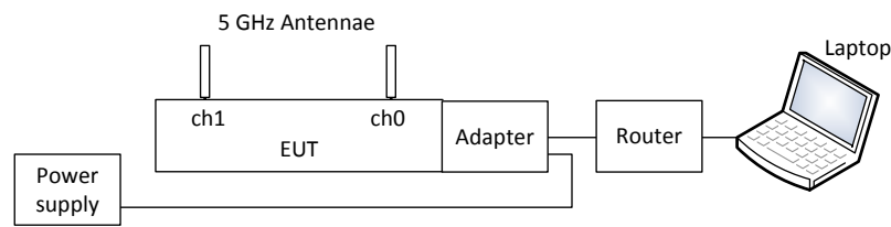
Figure 3.6-1: Setup diagram
