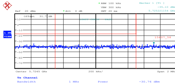
Figure 8.5-6: Lower band edge emissions at 5725 MHz, 802.11a, mid channel, cho
