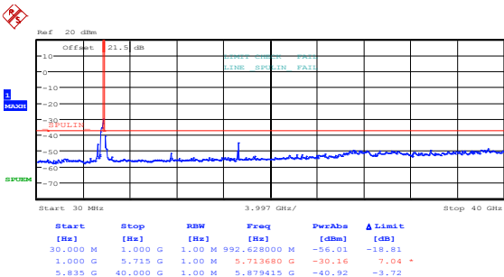
Figure 8.5-1: Conducted spurious emissions outside restricted bands, 802.11a, low channel, cho
