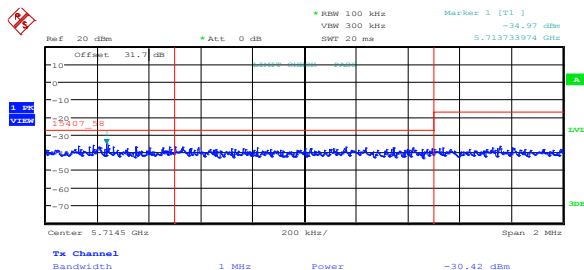
Figure 8.5-27: Lower band edge emissions at 5715 MHz, 802.11n HT20, mid channel, cho
