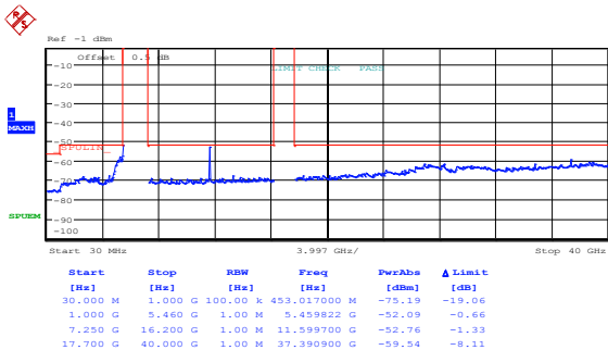
Figure 8.5-69: Conducted peak spurious emissions within restricted bands, 802.11a, high channel, cho
