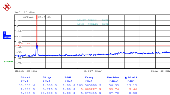
Figure 8.5-10: Conducted spurious emissions outside restricted bands, 802.11a, low channel, ch1
