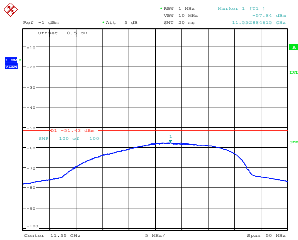
Figure 8.5-81: Conducted peak spurious emissions within restricted bands, 802.11n HT20, low channel, ch1
