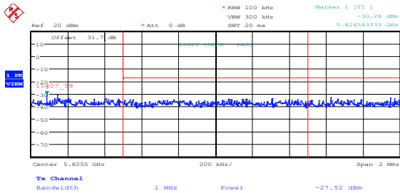
Figure 8.5-29: Upper band edge emissions at 5825 MHz, 802.11n HT20, mid channel, cho
