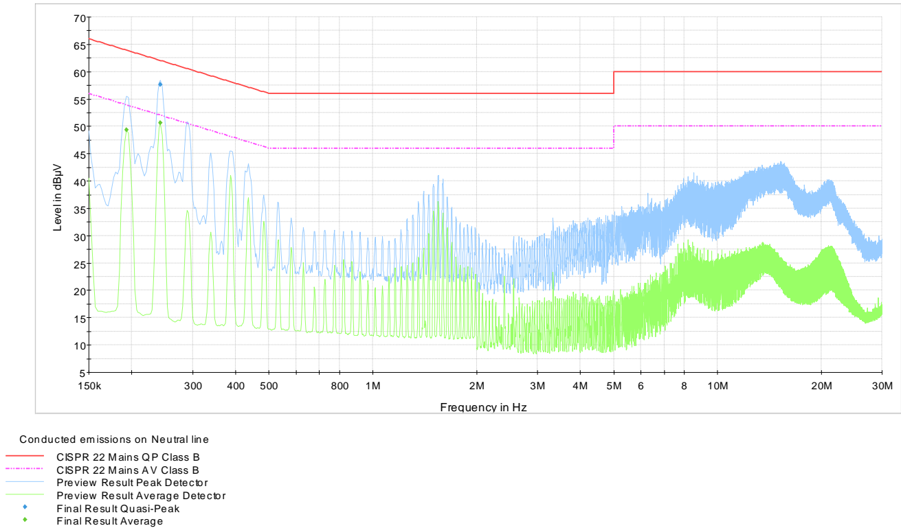
Figure 8.1-2: Conducted emissions on neutral line
