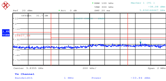
Figure 8.5-59: Upper band edge emissions at 5835 MHz, 802.11n HT40, low channel, ch1
