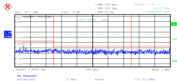
Figure 8.5-64: Upper band edge emissions at 5835 MHz, 802.11n HT40, high channel, ch1
