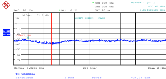
Figure 8.5-37: Upper band edge emissions at 5825 MHz, 802.11n HT20, low channel, ch1
