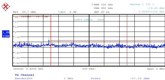
Figure 8.5-63: Upper band edge emissions at 5825 MHz, 802.11n HT40, high channel, ch1
