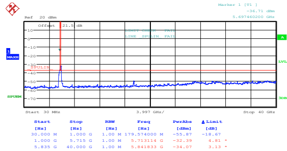
Figure 8.5-60: Conducted spurious emissions outside restricted bands, 802.11n HT40, high channel, ch1
