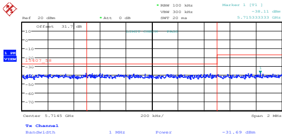
Figure 8.5-5: Lower band edge emissions at 5715 MHz, 802.11a, mid channel, cho
