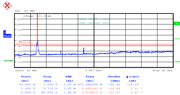
Figure 8.5-18: Conducted spurious emissions outside restricted bands, 802.11a, high channel, ch1
