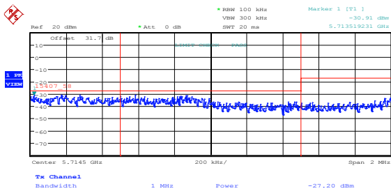
Figure 8.5-61: Lower band edge emissions at 5715 MHz, 802.11n HT40, high channel, ch1
