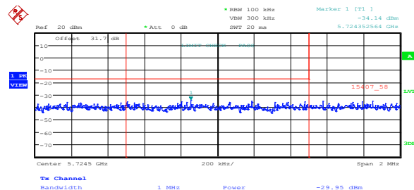
Figure 8.5-28: Lower band edge emissions at 5725 MHz, 802.11n HT20, mid channel, cho
