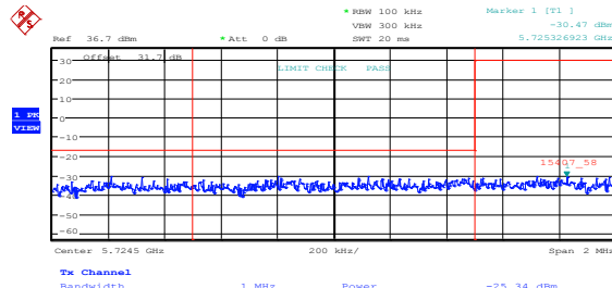
Figure 8.5-36: Lower band edge emissions at 5725 MHz, 802.11n HT20, low channel, ch1
