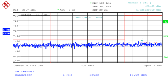
Figure 8.5-25: Lower band edge emissions at 5725 MHz, 802.11n HT20, low channel, cho
