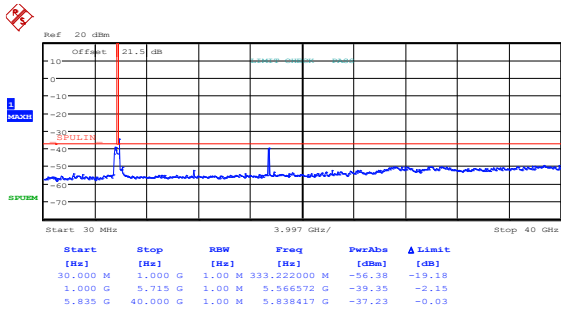
Figure 8.5-7: Conducted spurious emissions outside restricted bands, 802.11a, high channel, cho
