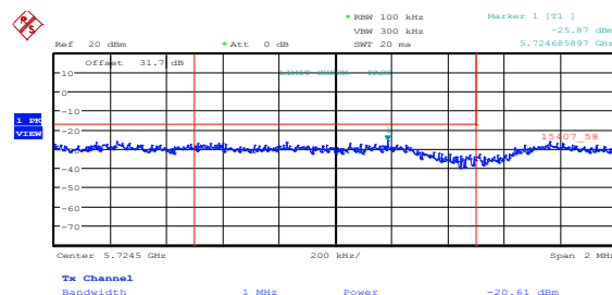
Figure 8.5-46: Lower band edge emissions at 5725 MHz, 802.11n HT20, high channel, ch1
