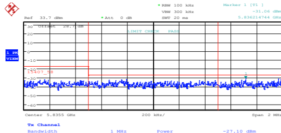
Figure 8.5-54: Upper band edge emissions at 5835 MHz, 802.11n HT40, high channel, cho
