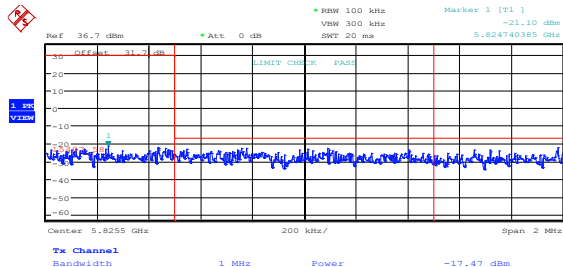
Figure 8.5-53: Upper band edge emissions at 5825 MHz, 802.11n HT40, high channel, cho
