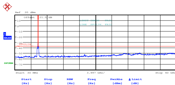
Figure 8.5-34: Conducted spurious emissions outside restricted bands, 802.11n HT20, low channel, ch1
