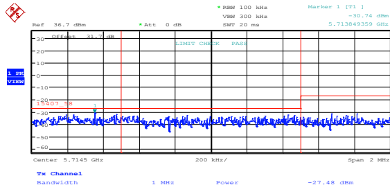
Figure 8.5-11: Lower band edge emissions at 5715 MHz, 802.11a, low channel, ch1
