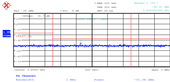
Figure 8.5-17: Upper band edge emissions at 5835 MHz, 802.11a, mid channel, ch1
