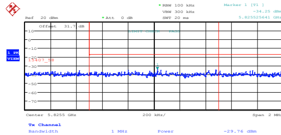
Figure 8.5-42: Upper band edge emissions at 5825 MHz, 802.11n HT20, mid channel, ch1
